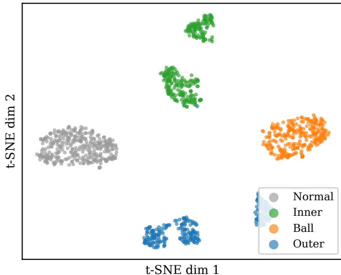
(b) With L_{\text{kin}} ( \lambda=0.01 , cover) Davies-Bouldin Index = 0.417
