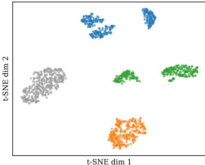
(a) Without L_{\text{kin}} Davies-Bouldin Index = 0.414
