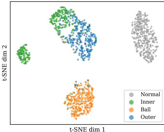
(b) With L_{\text{kin}} ( \lambda=0.01 , cover) Davies-Bouldin Index = 0.909
