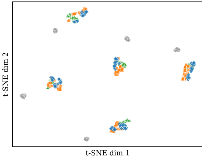
(a) Instantaneous Freq. Space (Epoch 1) Davies-Bouldin Index = 13.05
