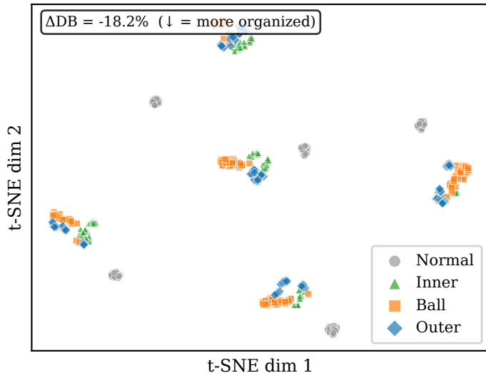
(b) Instantaneous Freq. Space (Epoch 50) Davies-Bouldin Index = 10.68
