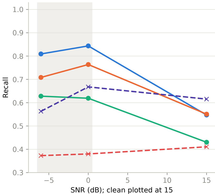
Inner-race (hard class)
