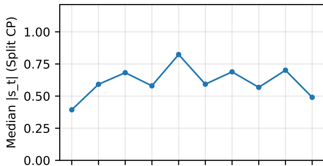
FD003
