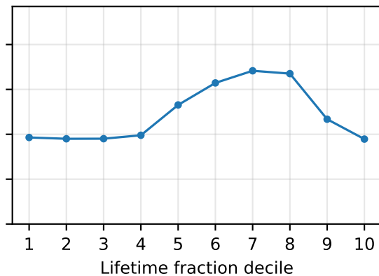
FD004
