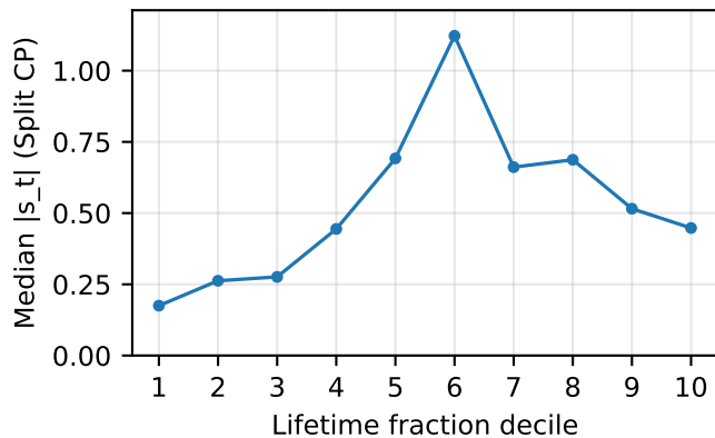
FD003
