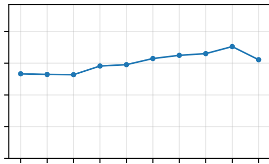
FD004
