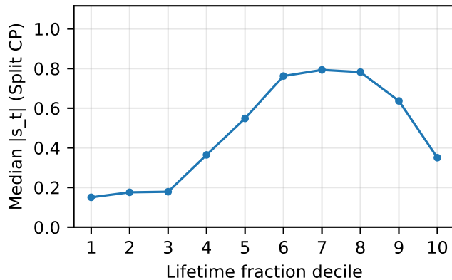
FD003
