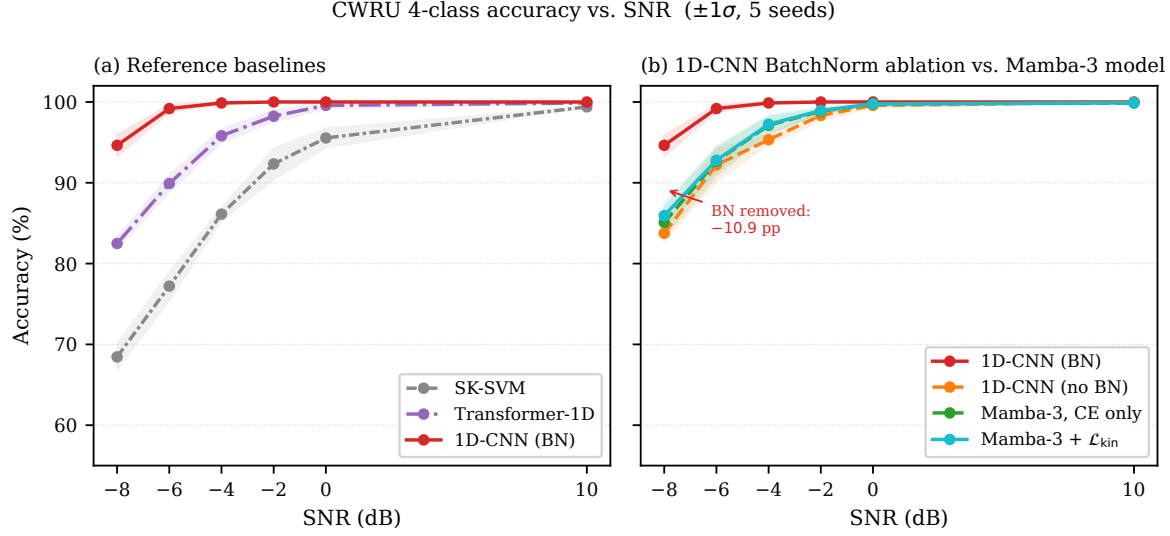
Figure A4. CWRU four-class DE accuracy against SNR ( \pm 1 SD, 5 seeds). The rightmost point of every curve, plotted at the 10 dB tick, is the no-noise (clean) run. (a) Reference baselines: SK-SVM, Transformer-1D and 1D-CNN (BN). (b) Removing all eight BatchNorm layers lowers the 1D-CNN from 94.64% to 83.76% at -8 dB ( \Delta = -10.88 pp); the Mamba-3 model, CE only (85.09%) and +\mathcal{L}_{kin} (85.94%), overlaps the no-BN curve ( p = 0.19 ). Replacing BatchNorm with GroupNorm(1, d) restores the within-condition accuracy (96.09% at -8 dB, table A12) but not the cross-condition result (table A13).
