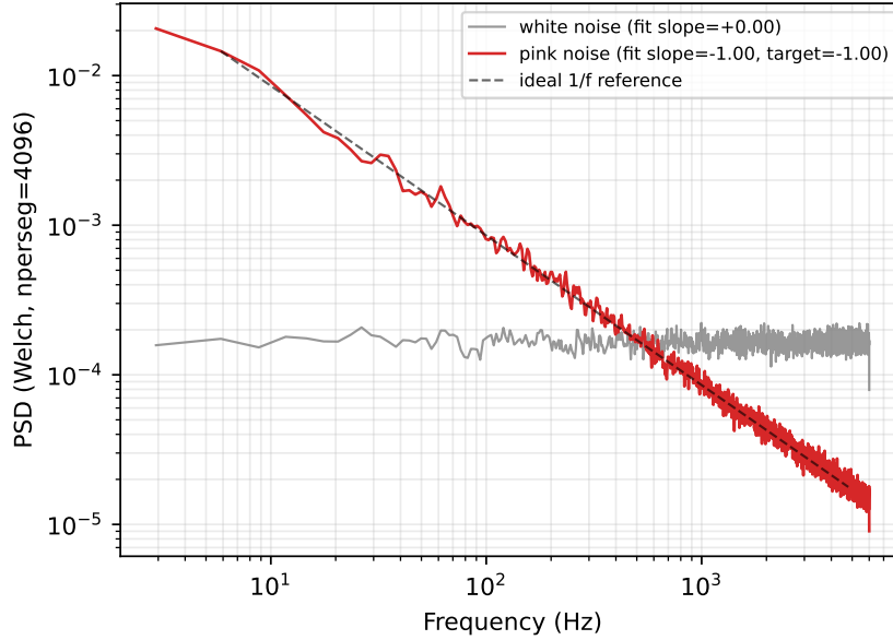
Pink vs white noise PSD — spectral verification of the pink-noise generator
