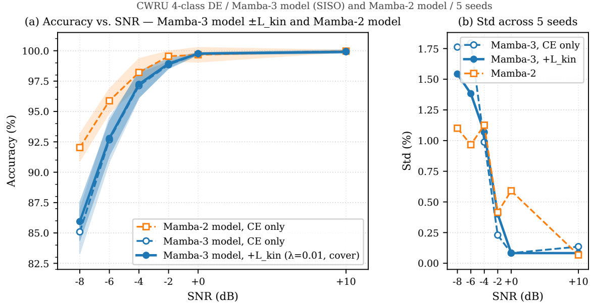
Figure A5. CWRU four-class DE test accuracy (a) and inter-seed SD (b) against SNR, leakage-free protocol, for the Mamba-2 model (CE only) and the Mamba-3 model, CE only and +\mathcal{L}_{\text{kin}} ( \lambda = 0.01 , 5 seeds). (a) The Mamba-2 model is higher at -6 and -8 dB ( p = 0.063 , two-sided) and marginally at -4 dB ( p = 0.19 ); \mathcal{L}_{\text{kin}} neither shifts the mean curve nor consistently narrows the SD band relative to CE only. (b) The inter-seed SD with \mathcal{L}_{\text{kin}} changes in both directions across the SNR grid (table A16).
