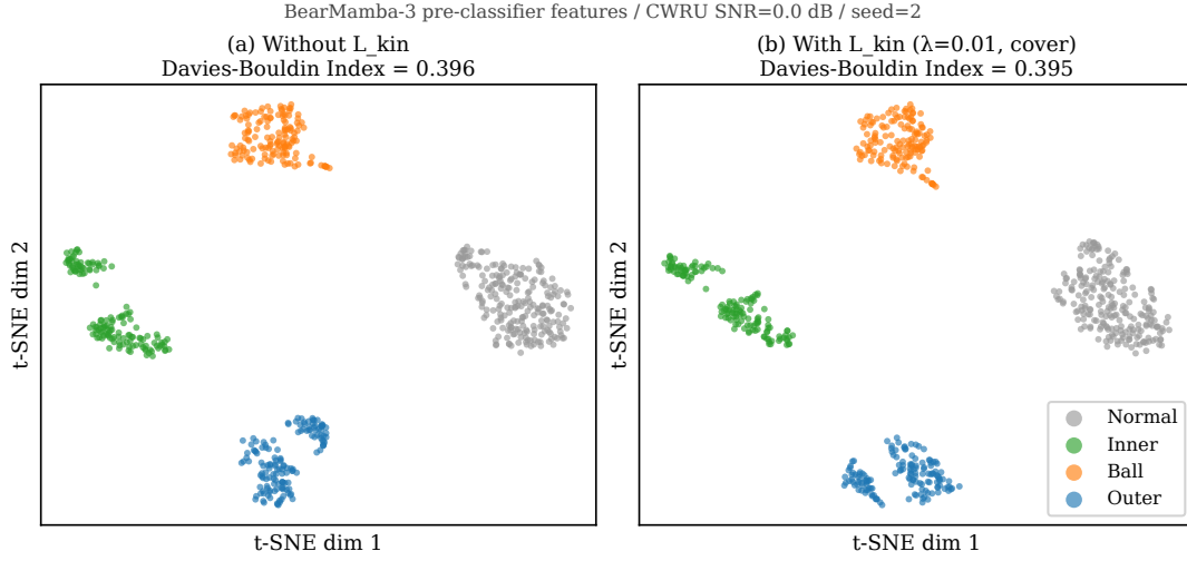
Figure A9. t-SNE of pre-classifier features, Mamba-3 model, CWRU DE, SNR = 0 dB, seed 2. (a) CE only: DB = 0.396, four well-separated clusters. (b) +\mathcal{L}_{\text{kin}} ( \lambda = 0.01 ): DB = 0.395, nearly identical cluster geometry. The pre-classifier feature space is near ceiling at this SNR, which is consistent with the non-significant difference in mean accuracy (one-sided p = 0.6875^\dagger at 0 dB, table A16). The figure title uses the earlier name “BearMamba-3” for the Mamba-3 model.
