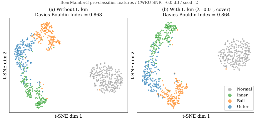
Figure A10. t-SNE of pre-classifier features, CWRU DE, Mamba-3 model, SNR = -6 dB, seed 2, leakage-free protocol. (a) CE only: DB = 0.868; (b) +\mathcal{L}_{kin} : DB = 0.864. At this noise level the fault-class clusters overlap substantially in both cases; \mathcal{L}_{kin} does not recover separability. The two DB values differ by less than the inter-seed range and do not indicate a stable direction (figure A11). The figure title uses the earlier name “BearMamba-3” for the Mamba-3 model.
