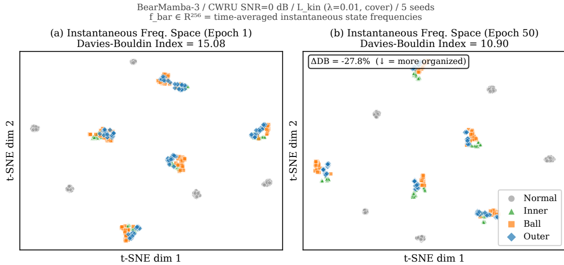
Figure A8. t-SNE of the time-averaged state frequencies \bar{\mathbf{f}} \in \mathbb{R}^{256} at epoch 1 (a) and epoch 50 (b), Mamba-3 model, CWRU DE, SNR = 0 dB, +\mathcal{L}_{\text{kin}} ( \lambda = 0.01 , cover), 5 seeds (320 samples plotted). Each point is a vibration window; colours denote fault classes. The Davies–Bouldin index decreases from 15.08 to 10.90 ( \Delta = -27.8\% ; lower is more compact). This describes the state-frequency space only; compare figure A9, which shows that the pre-classifier feature space is already well separated without \mathcal{L}_{\text{kin}} at this SNR. The figure title uses the earlier name “BearMamba-3” for the Mamba-3 model, and the panel annotation’s “more organized” means a lower DB index (more compact clusters).
