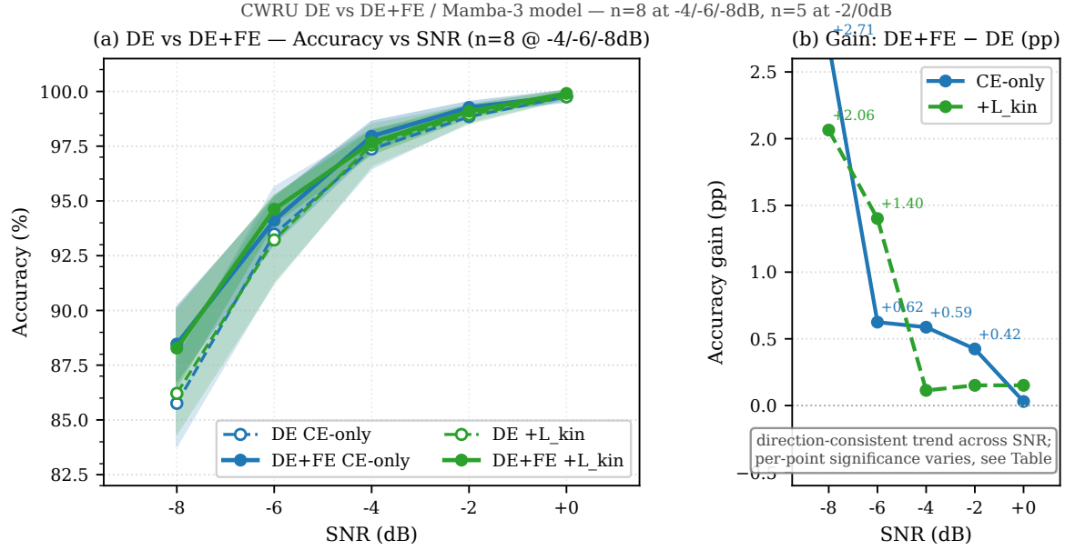
Figure A3. CWRU DE and DE+FE accuracy of the Mamba-3 model against SNR ( \pm 1 SD shaded; n = 8 seeds at -4 , -6 and -8 dB, n = 5 at -2 and 0 dB; first software environment). (a) Accuracy: solid, DE+FE; dashed, DE; blue, CE only; green, +\mathcal{L}_{\text{kin}} . (b) DE+FE minus DE (pp); per-point p values (nominal, one-sided, not adjusted for multiplicity) are in table A4.
