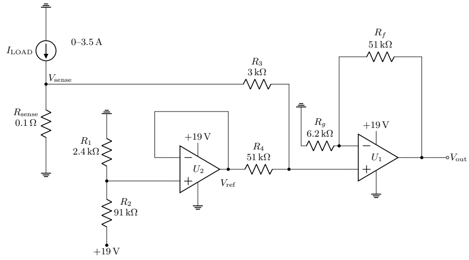
Figure 1: Candidate Design 2: buffered reference and weighted non-inverting amplifier.
