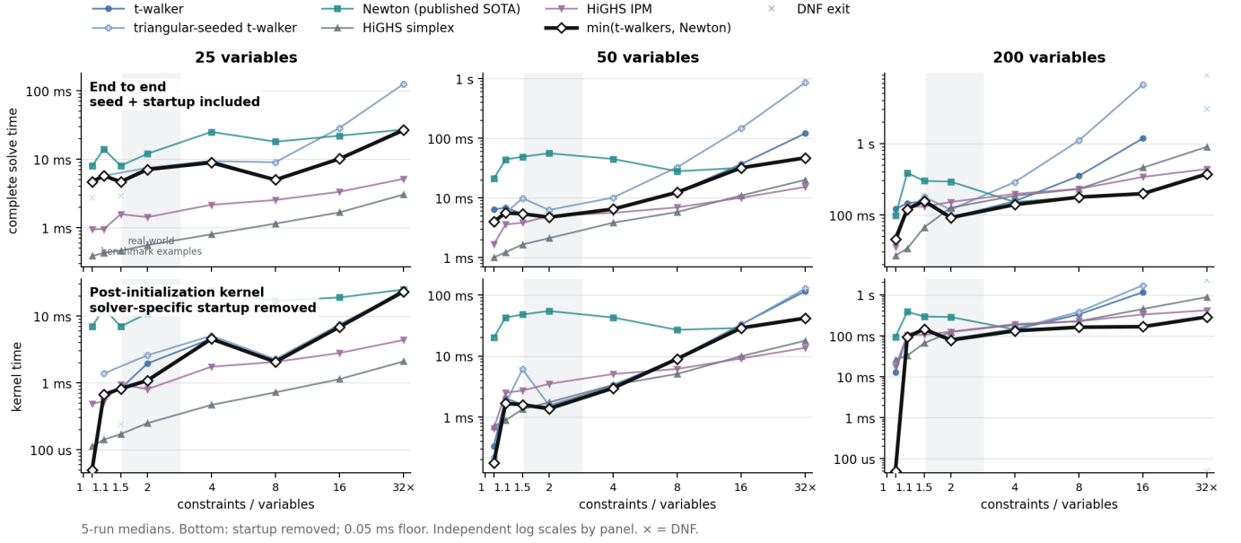
Figure 1: Complete time above and post-initialization kernel time below. The black line shows the fastest certified default-seed walker, triangular-seeded walker, or Newton result. The measured axis starts at 1.1; we retain 1.0 only as a reference. The generator changes aspect ratio and planted support geometry together, so the plot establishes a useful regime, not a theorem that aspect ratio alone is causal.
