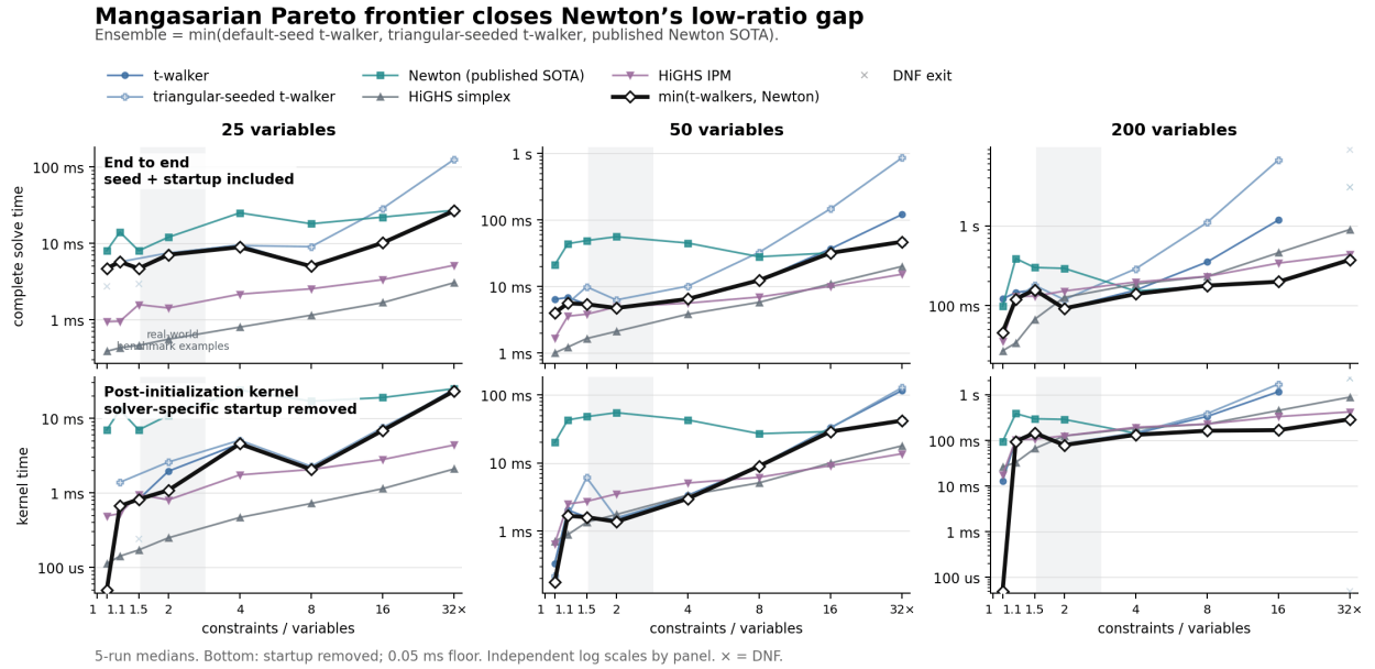
Figure 1: Complete time above and post-initialization kernel time below. The black line shows the fastest certified default-seed t-walker, triangular-seeded t-walker, or Newton result. The measured axis starts at 1.1; we retain 1.0 only as a reference. The generator changes aspect ratio and planted support geometry together, so the plot establishes a useful regime, not a theorem that aspect ratio alone is causal.
