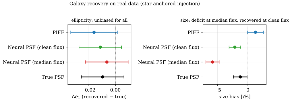
Figure 8. Galaxy recovery on real data (star-anchored injection), median \pm bootstrap 95% CI per PSF. Left: recovered ellipticity is low-bias ( |\Delta e_1| \lesssim 0.016 ) for all three methods. Right: recovered size . Queried at the median flux our model runs small (contamination-broadening of the predicted PSF); queried at the clean high-flux limit it recovers to near the true-PSF floor (§4.4). PIFF is shown for reference.
