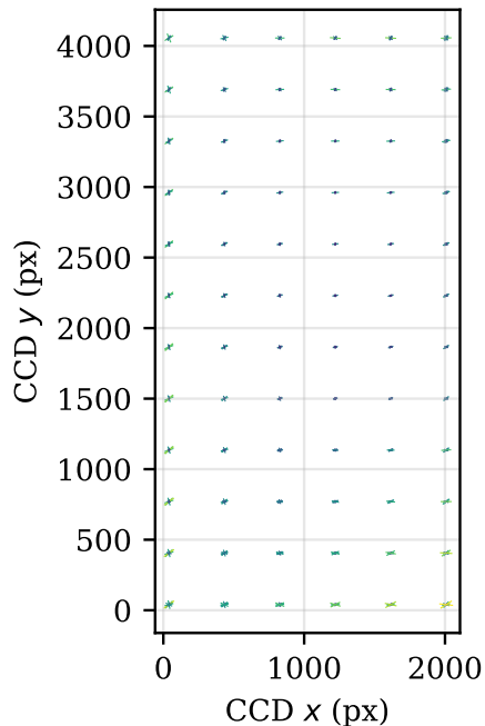
Figure 4. The true, spatially varying PSF ellipticity field in a simulated exposure (whisker length \propto |e| ); the network must recover this at star-free positions.
