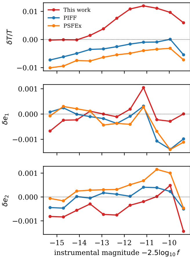
Residuals vs magnitude (brighter-fatter)
