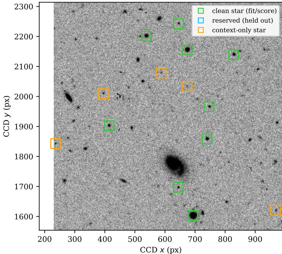
DES single-epoch r -band (CCD 31), star selection
