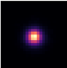
PSFEx
