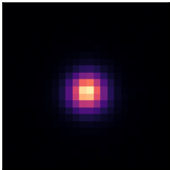
observed star
