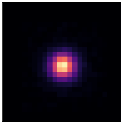
PIFF
