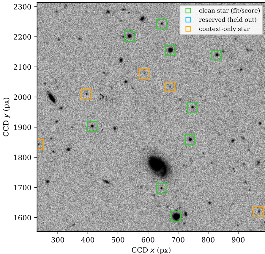
DES single-epoch r -band (CCD 31), star selection
