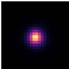
observed star
