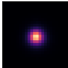
Neural PSF
