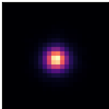
PSFEx
