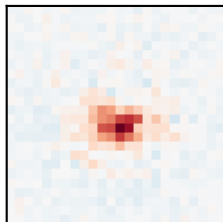
PSFEx residual
