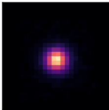
PIFF
