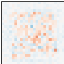
PIFF residual
