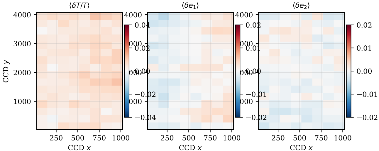
Neural PSF residual maps across the CCD
