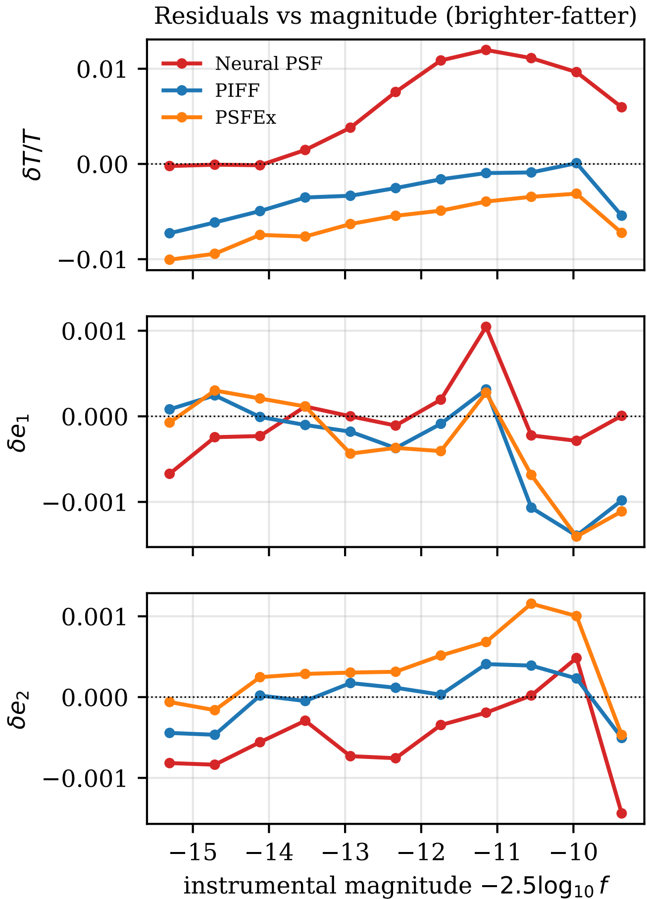
Figure 14. Residuals versus instrumental magnitude (cf. PIFF Fig. 10). Our model (red) carries a magnitude-dependent size residual peaking at \pm 1.2\% (85).
