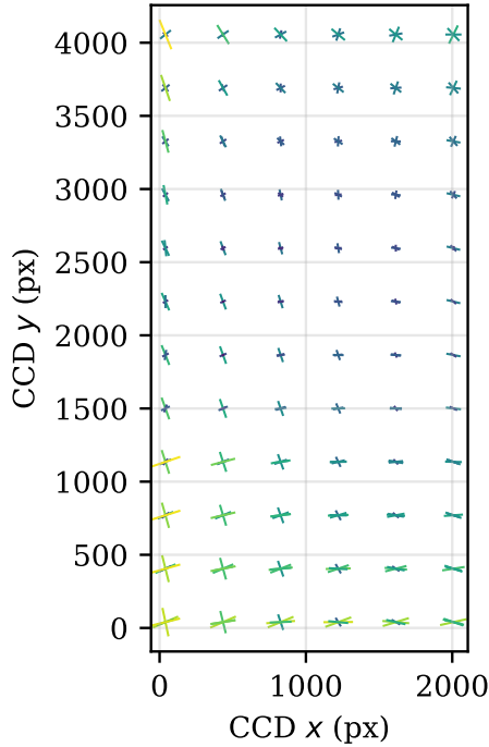
True PSF ellipticity field (simulation)
