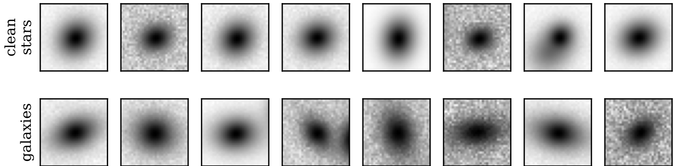
Figure 3. Example simulated cutouts. Clean stars (top) are compact point sources; injected galaxies (bottom) are visibly extended and elliptical (second-moment size T \approx 33 vs 15 px 2 ). Both are presented to the network as context.
