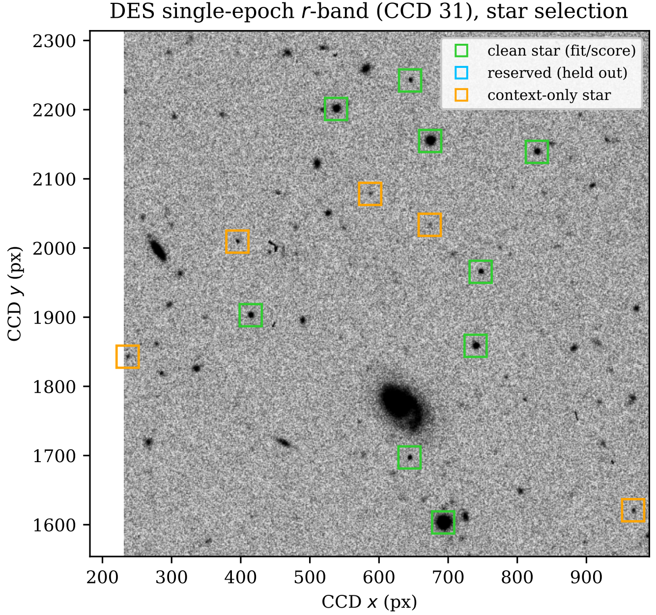
Figure 10. Star selection on a real DES exposure. Green: clean stars (fit and score). Blue: reserved (held out for evaluation). Orange: context-only stellar detections. Extended sources (galaxies) are excluded from the attention context.
