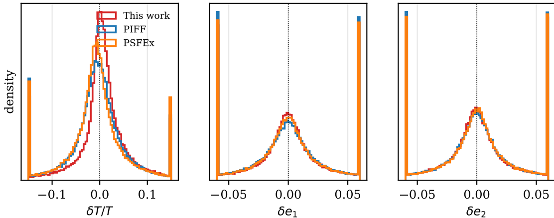
Reserved-star residuals on the DES test split
