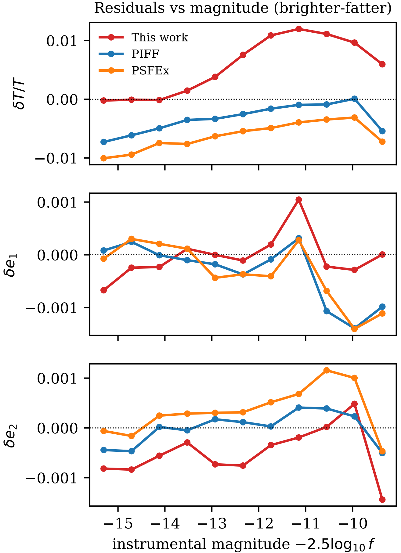
Figure 13. Residuals versus instrumental magnitude (cf. PIFF Fig. 10). Our model (red) carries a magnitude-dependent size residual peaking at +1.2\% (85).
