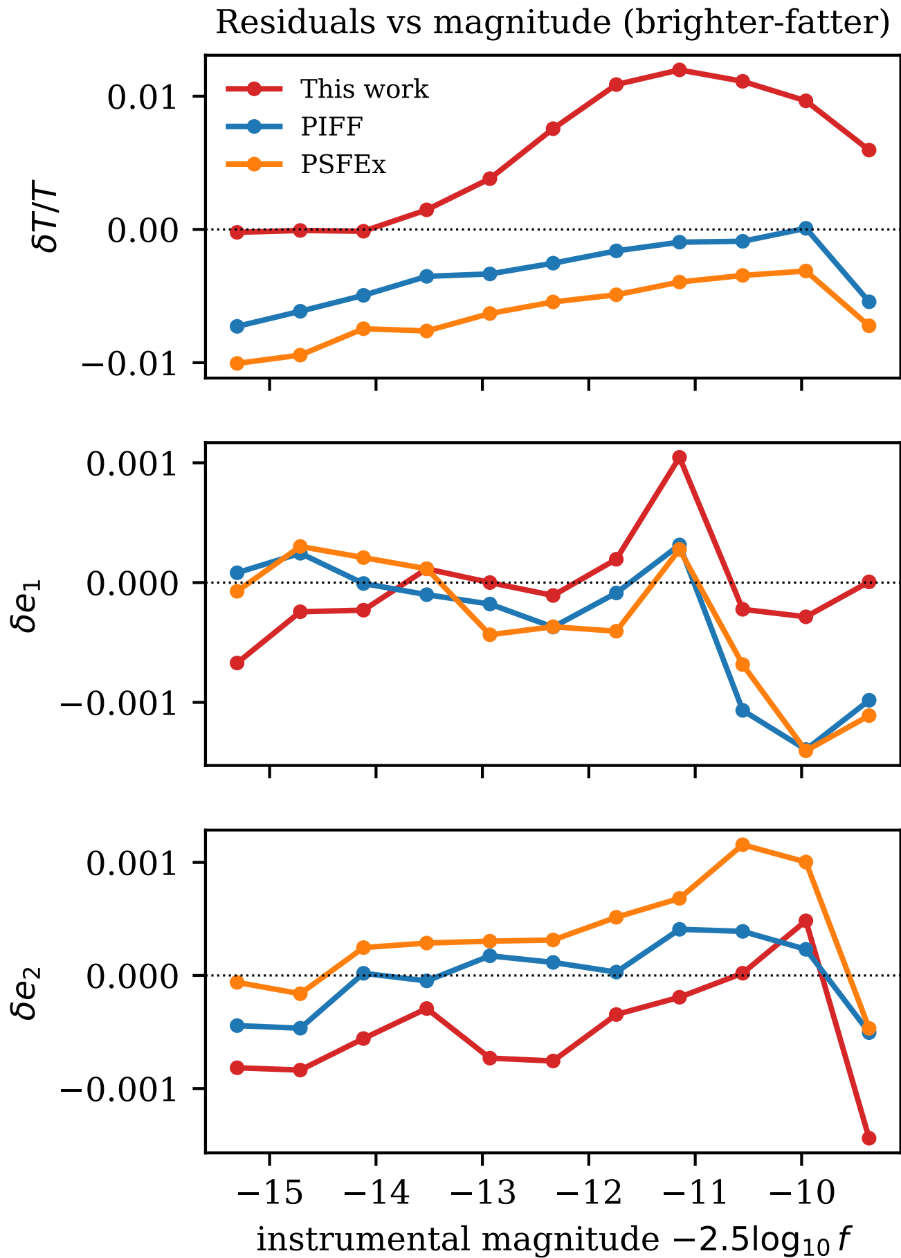
Figure 14. Residuals versus instrumental magnitude (cf. PIFF Fig. 10). Our model (red) carries a magnitude-dependent size residual peaking at +1.2\% (85).
