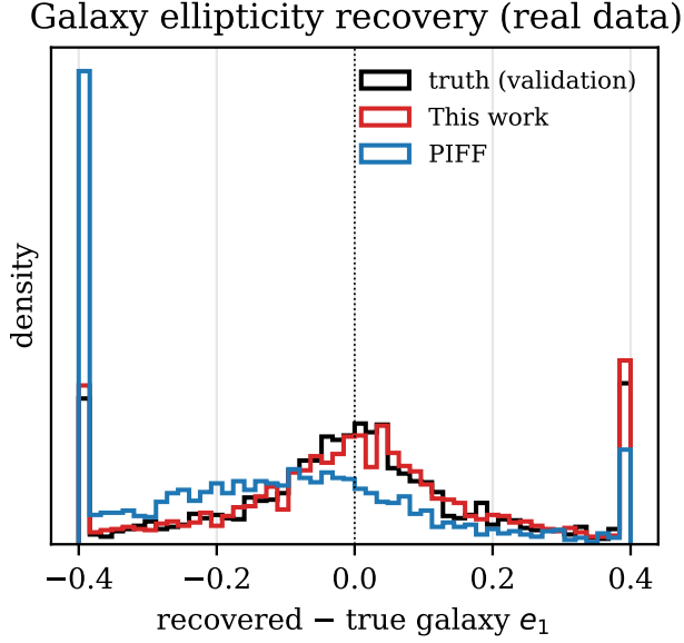
Figure 8. Galaxy ellipticity recovery on real data (star-anchored injection). PIFF’s PSF-ellipticity error biases recovered galaxy e_1 by -0.14 ; ours is unbiased.
