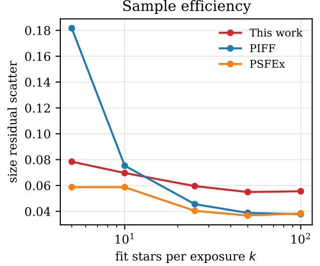
Figure 9. Size-residual scatter versus the number of fit stars k . The amortized model is nearly flat in k ; PIFF degrades sharply below k \approx 25 .
