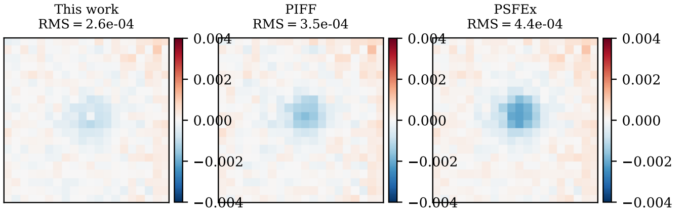
Figure 6. Stacked normalized pixel residual (observed star – model, unit-sum) over 306 reserved test stars, on a common scale. Our amortized model leaves the flattest residual; the per-exposure baselines retain a coherent central core—a higher-order shape error that second-moment metrics do not capture (§4.2).
