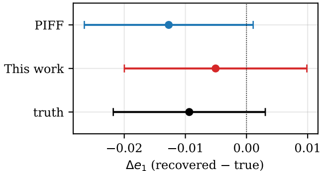
ellipticity: unbiased for all
