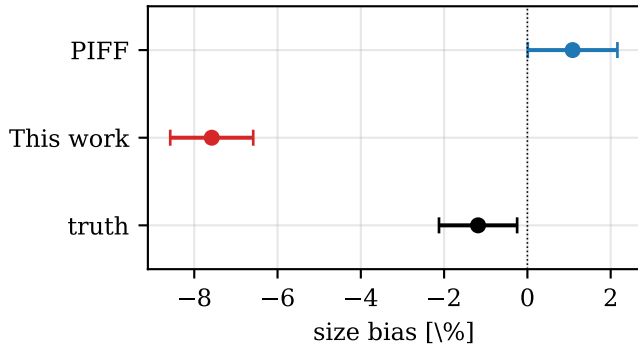
size: our model \sim 8\% small
