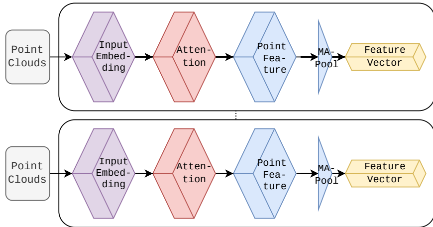
Point Cloud Feature Extraction Blocks
