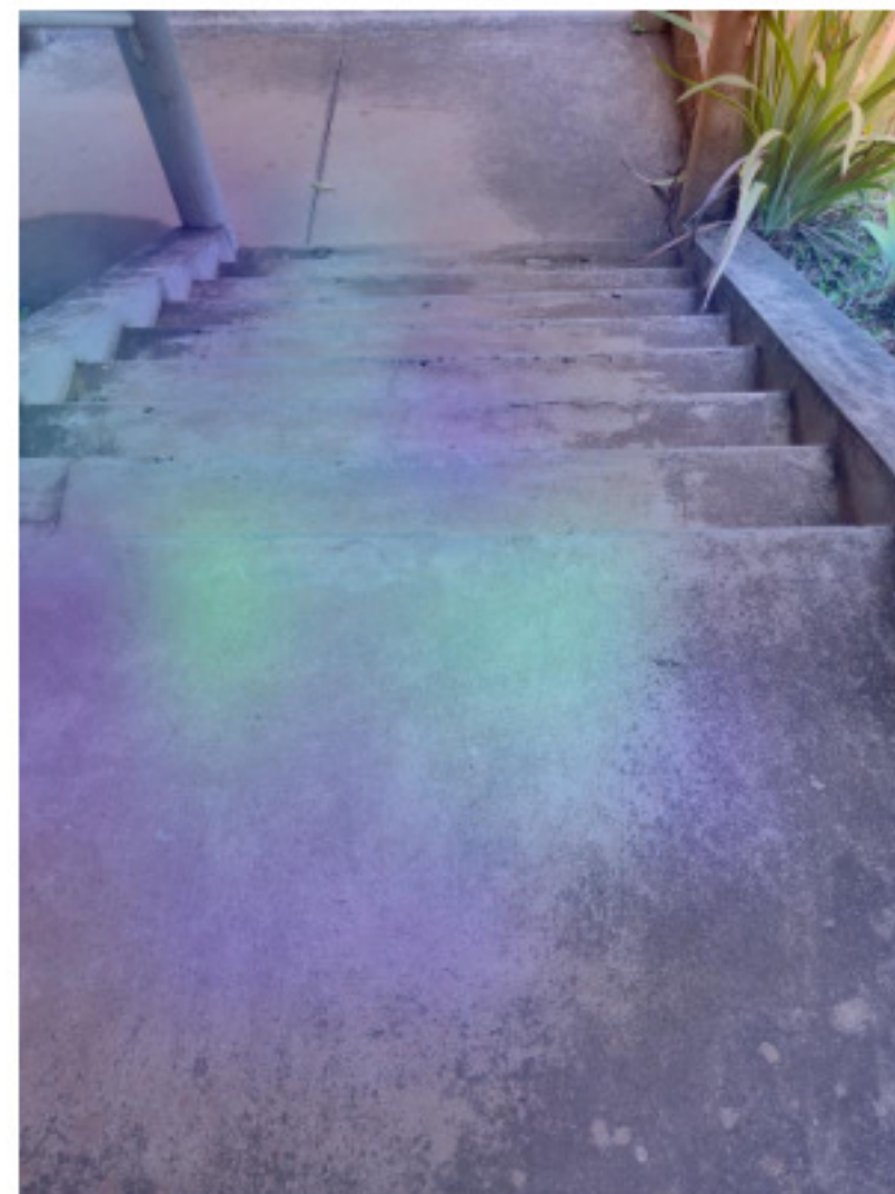
ResNet50
