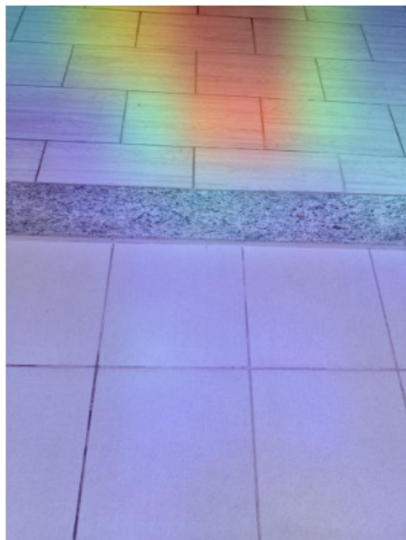
EfficientNetB0
