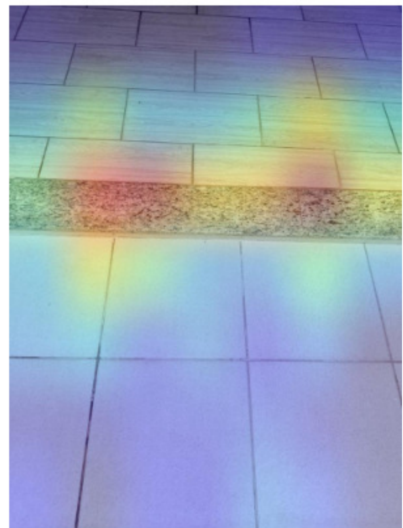
ResNet50
