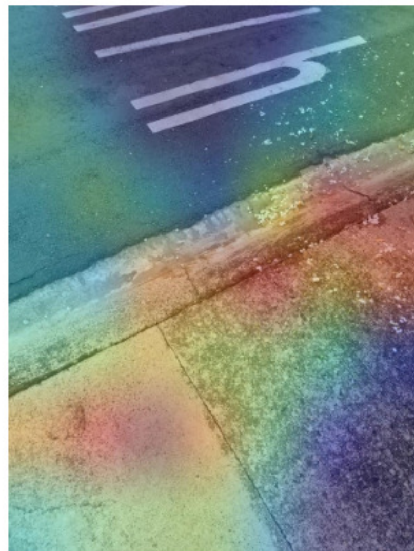
ResNet50
