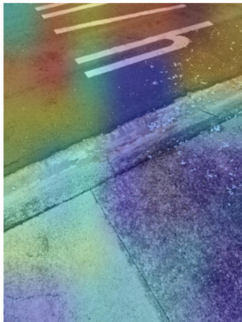
MobileNet
