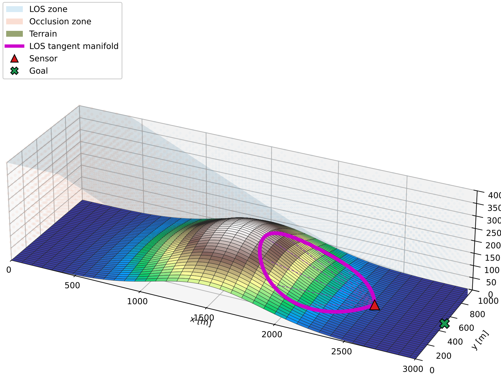
A 3D LOS and terrain-occlusion geometry
