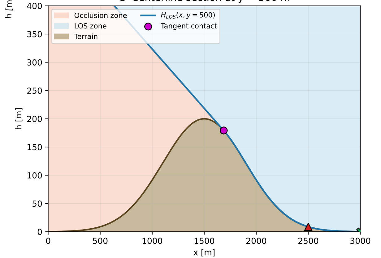
C Centerline section at y = 500 m
