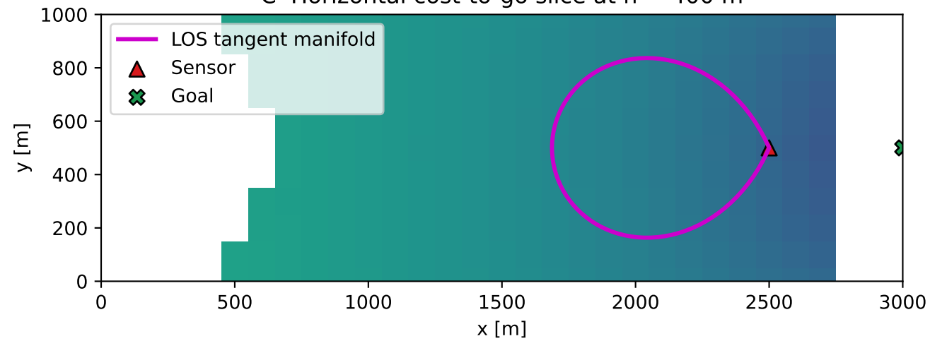
C Horizontal cost-to-go slice at h = 400 m
