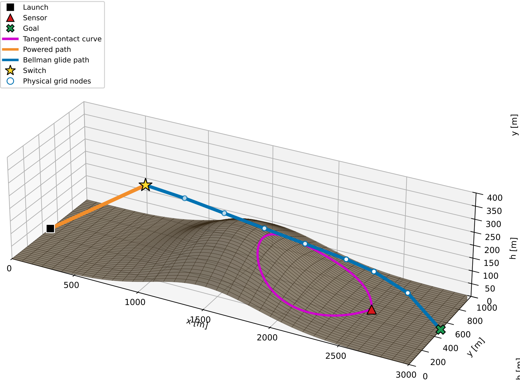
A Extracted physical Bellman trajectory
