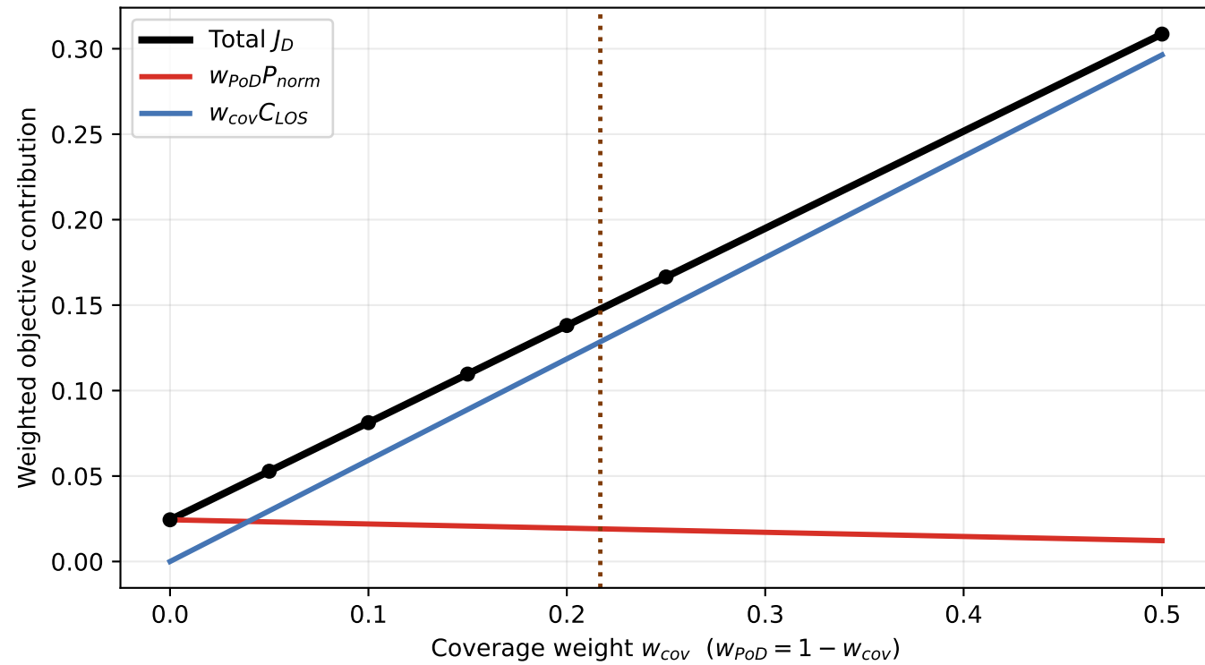
A Fixed center sensor: objective decomposition (2500, 500, 8.79 m): P_{norm}=0.02440 , C_{LOS}=0.59275
