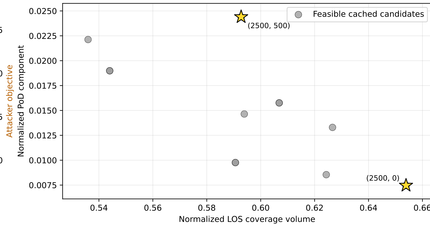
D Cached candidate tradeoff
