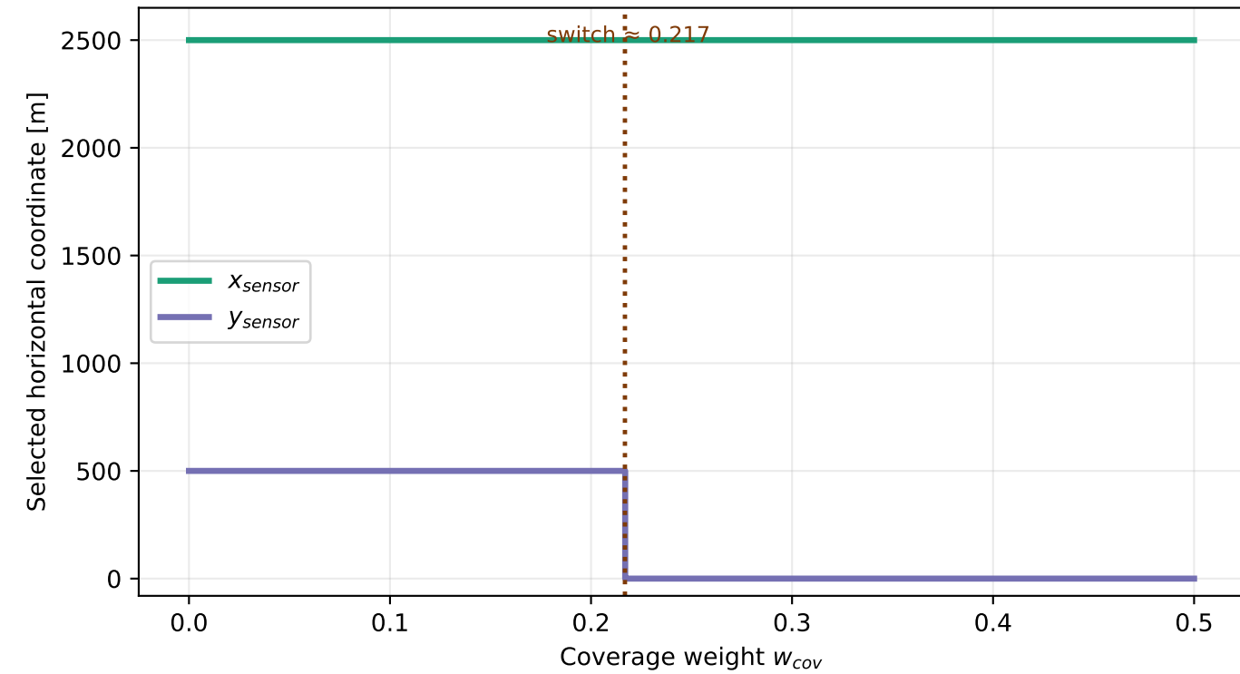
B Best cached sensor candidate
