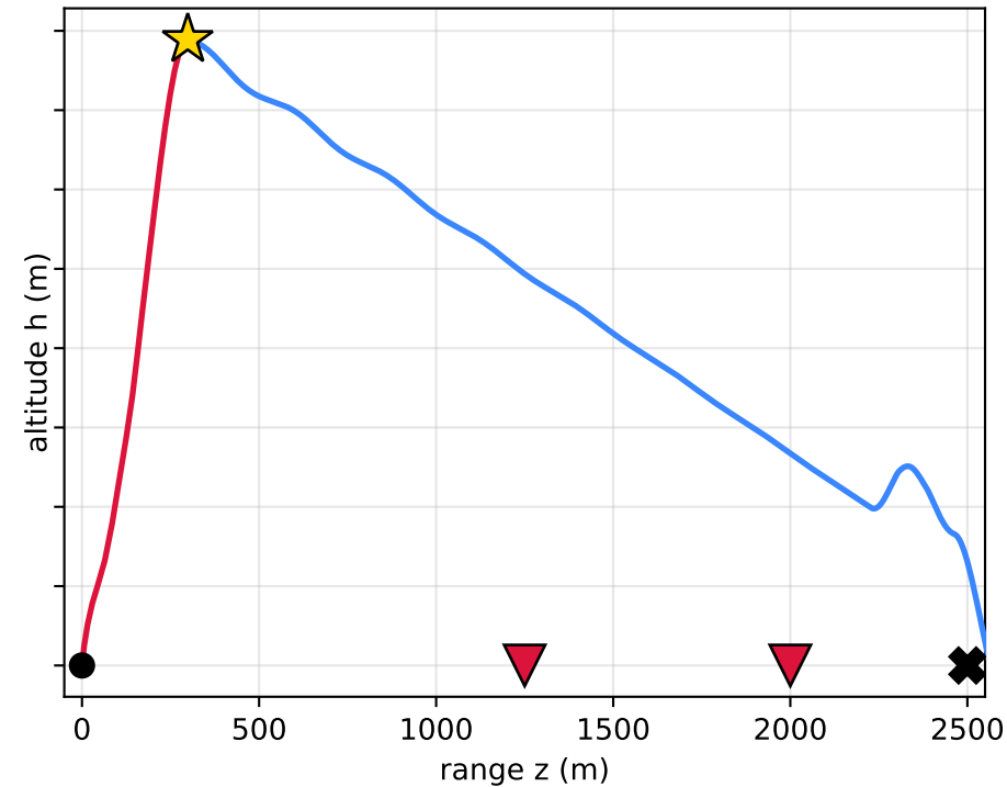
Greedy
