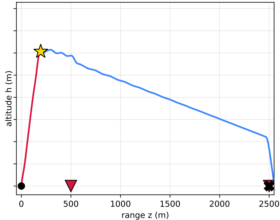
Naive
