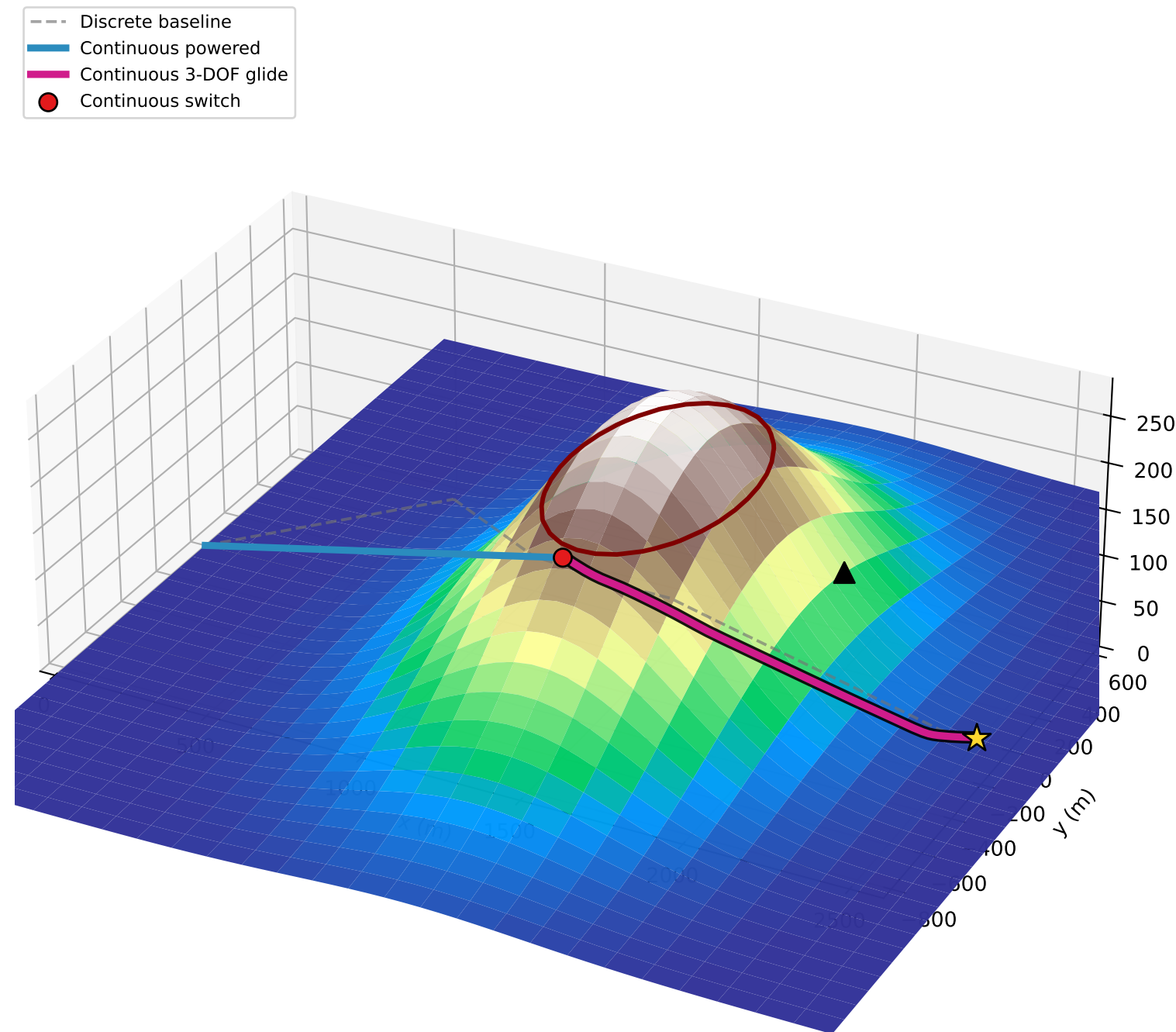
Continuous 3-DOF trajectory
