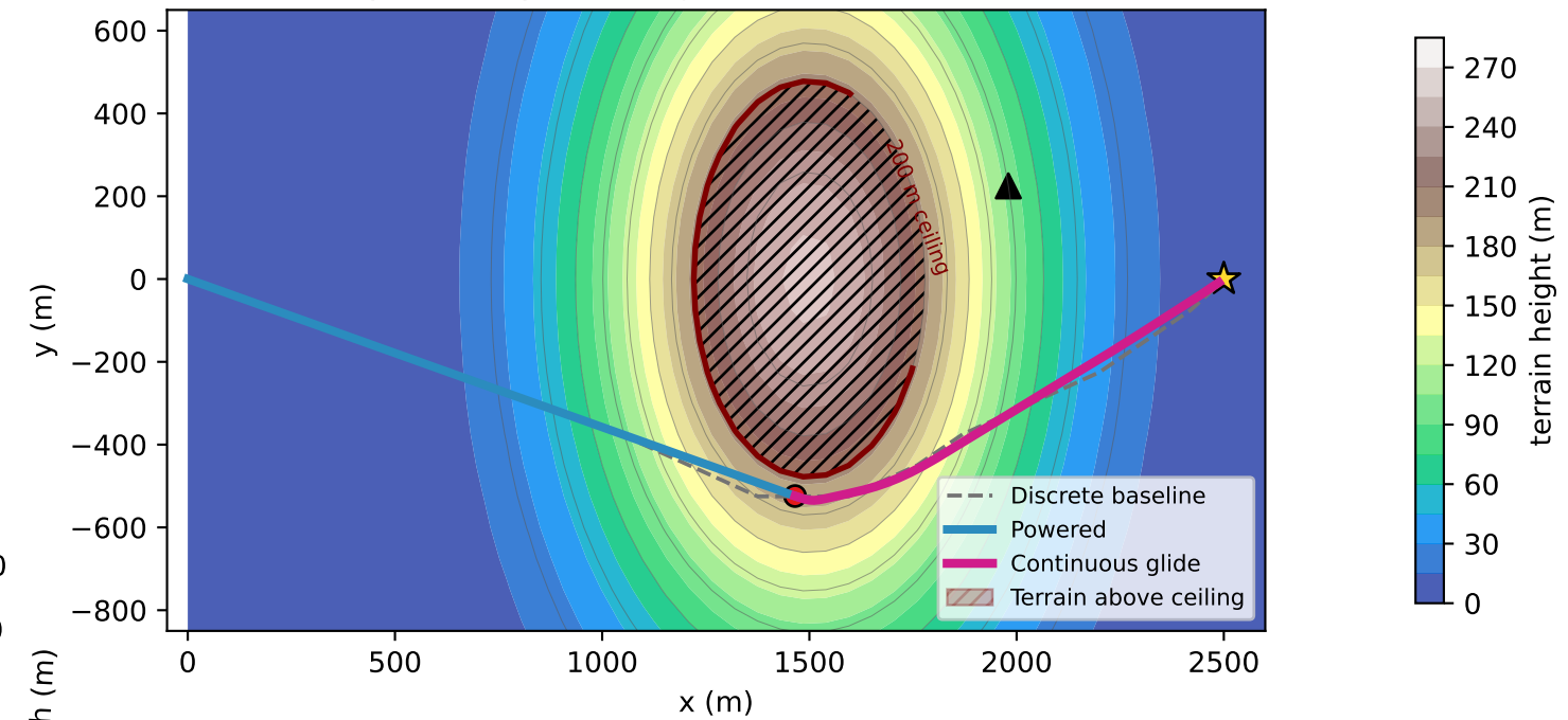
Continuous state history across the switch
