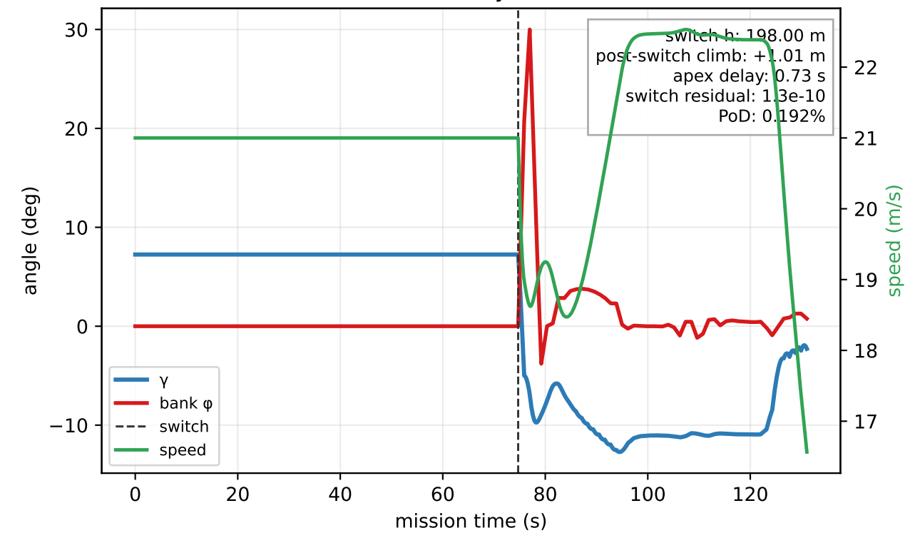
Continuous state history across the switch
