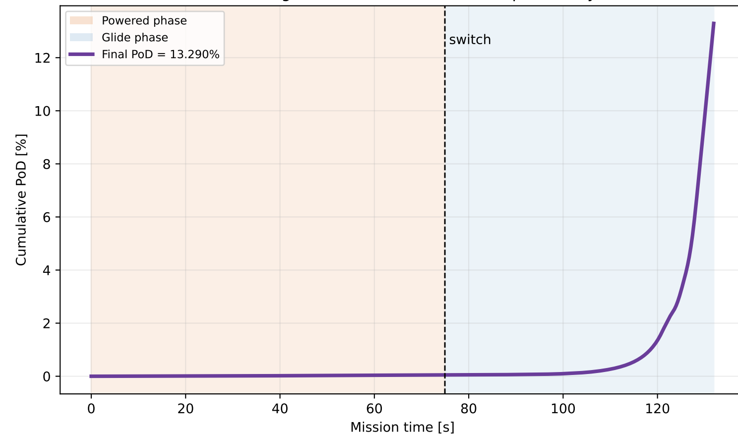
D Reintegrated cumulative detection probability
