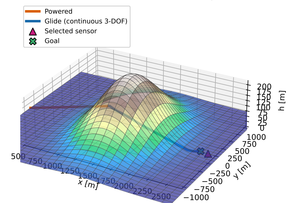
B Fine + continuous validated best response
