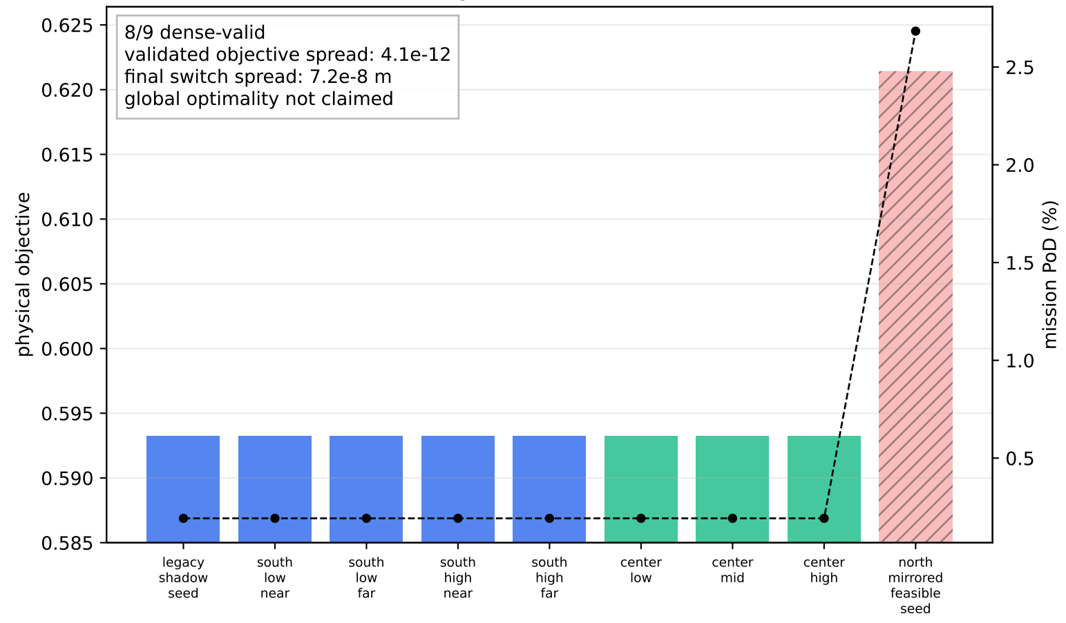
D. Basin ranking; hatched north solve is invalid
