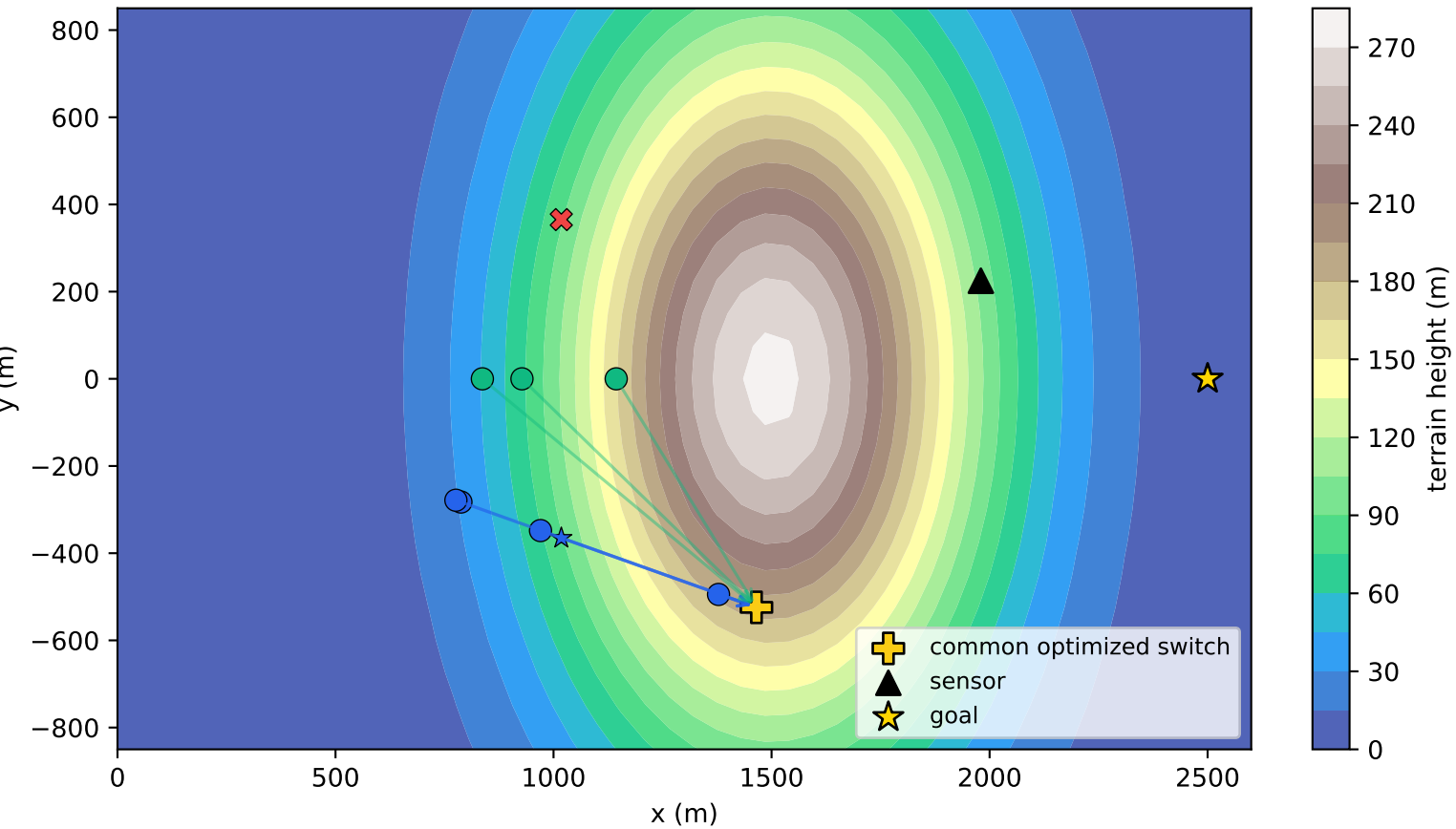
C. Eight validated trajectories overlap
