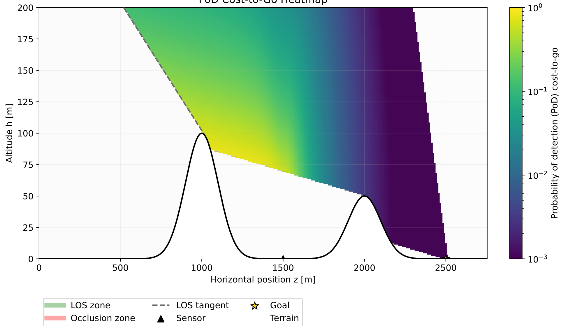
PoD Cost-to-Go Heatmap
