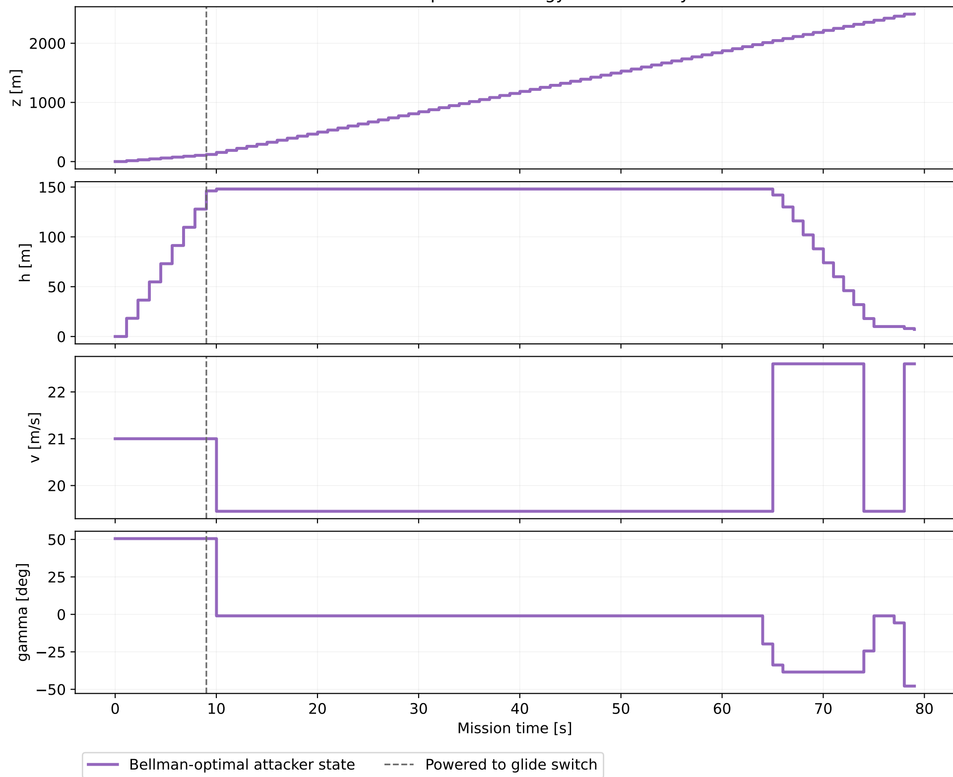
Attacker Optimal Strategy: State History
