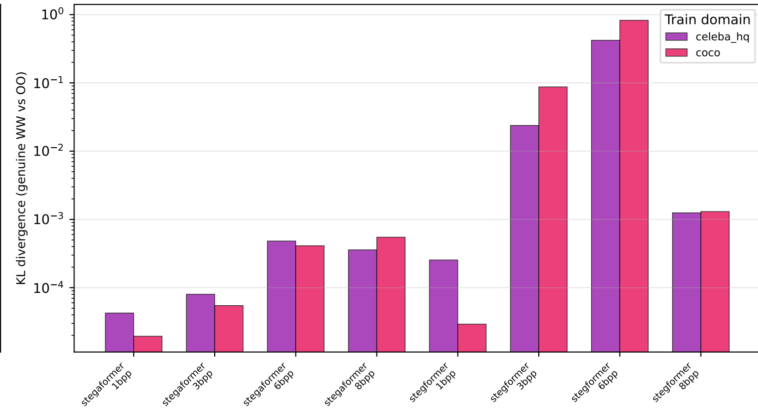
Arcface — offline
