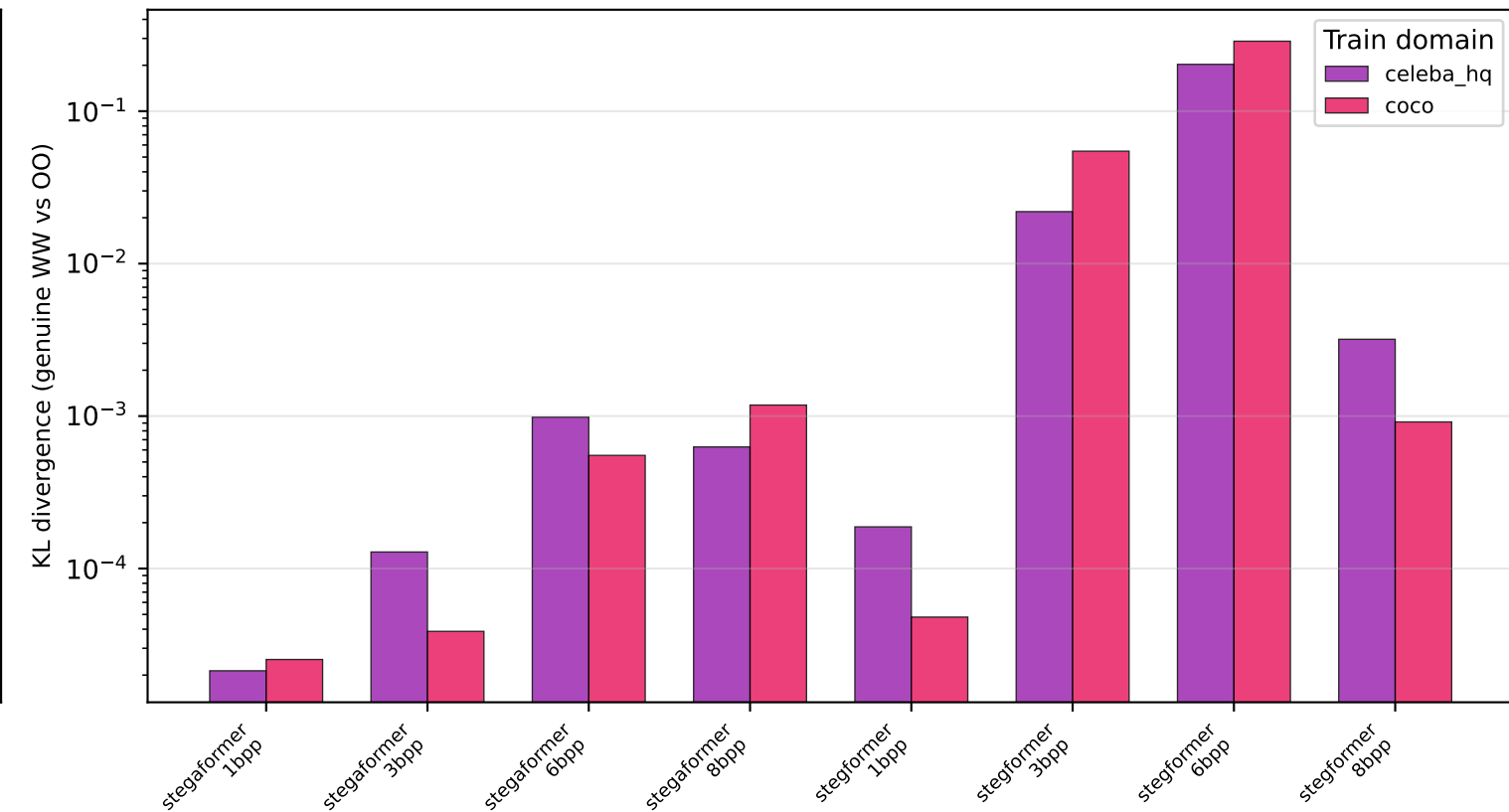
Facenet — offline
