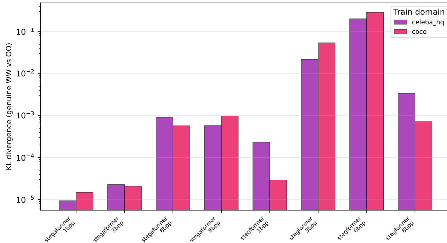
Facenet — online
