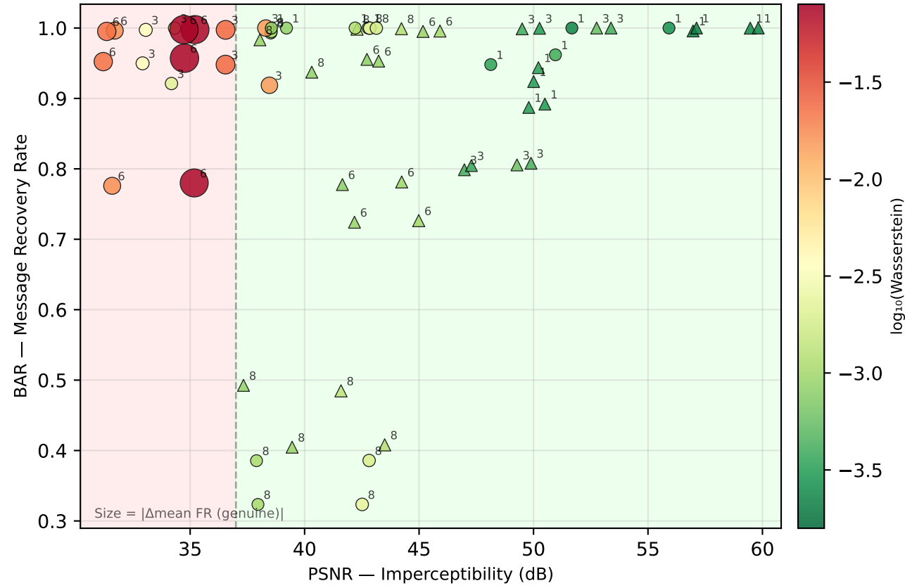
Arcface — WW
