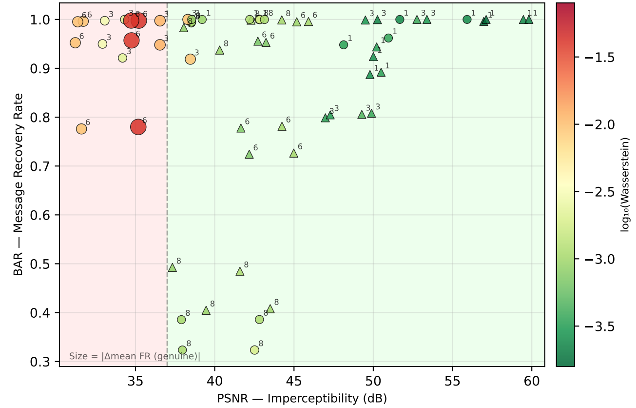
Facenet — WW
