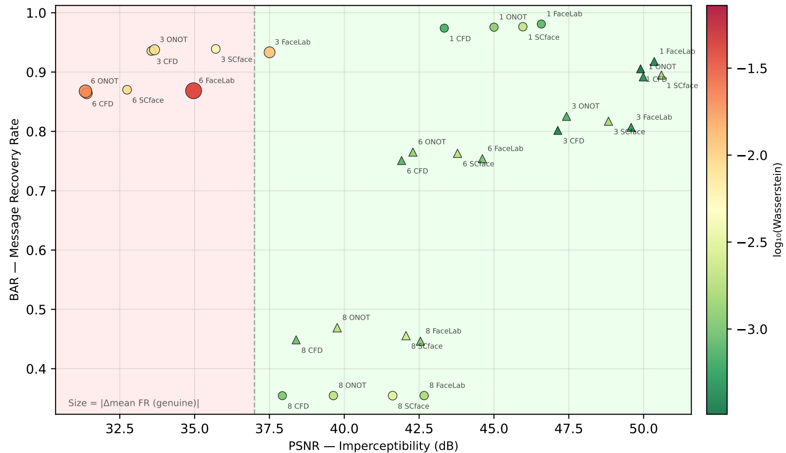
Watermarking Algorithm
