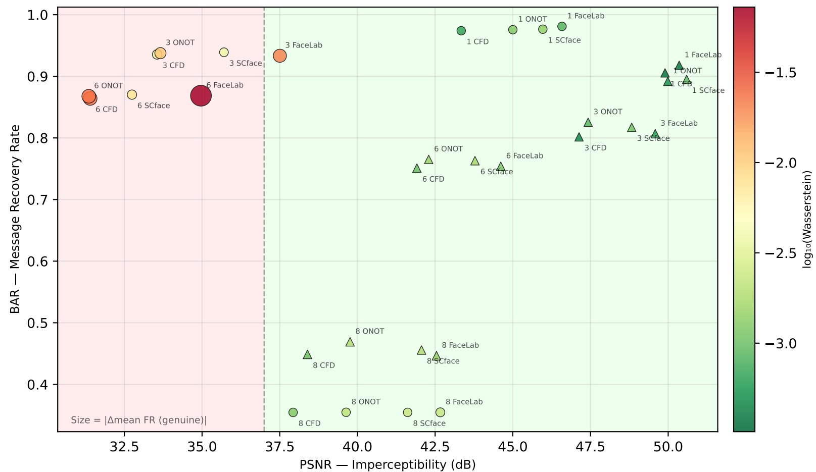
Facenet
