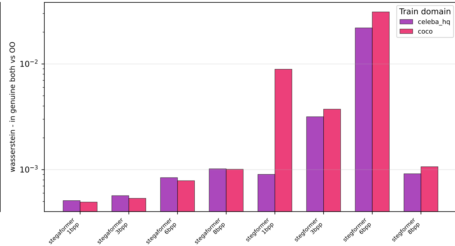
Arcface — offline
