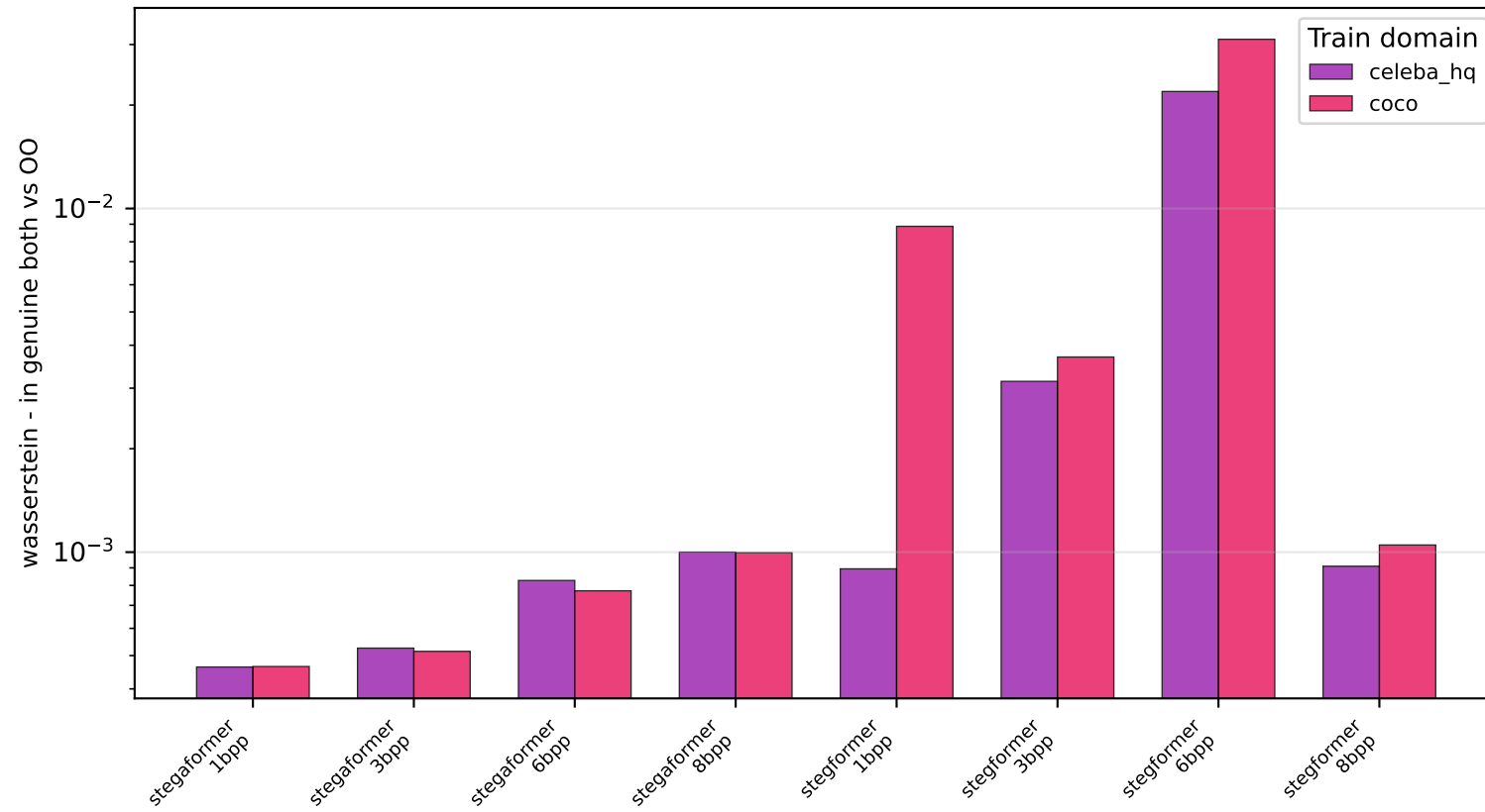
Arcface — online
