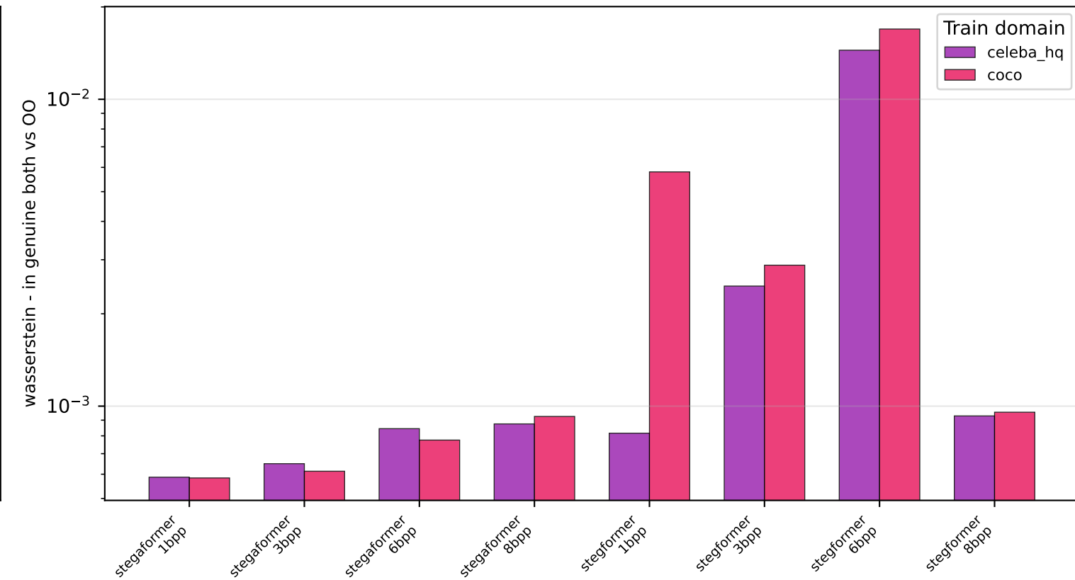
Facenet — offline
