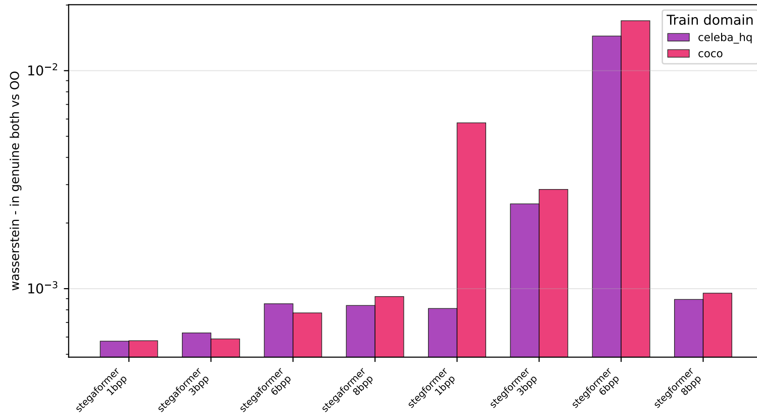
Facenet — online
