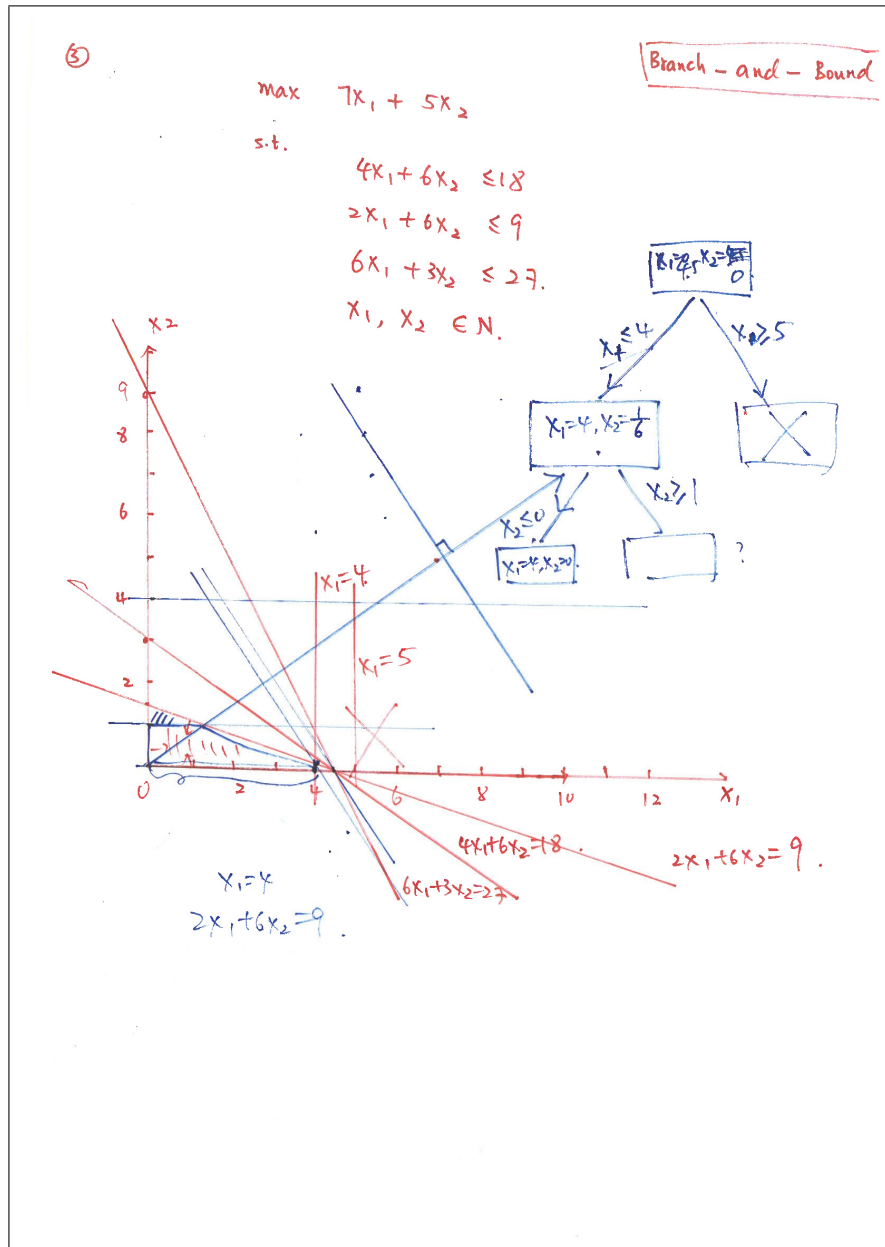
Figure 3: Q3 branch and bound: max 7x_1 + 5x_2 s.t. 4x_1 + 6x_2 \leq 18 , 2x_1 + 6x_2 \leq 9 , 6x_1 + 3x_2 \leq 27 , integer \Rightarrow (4, 0) , z = 28 .
