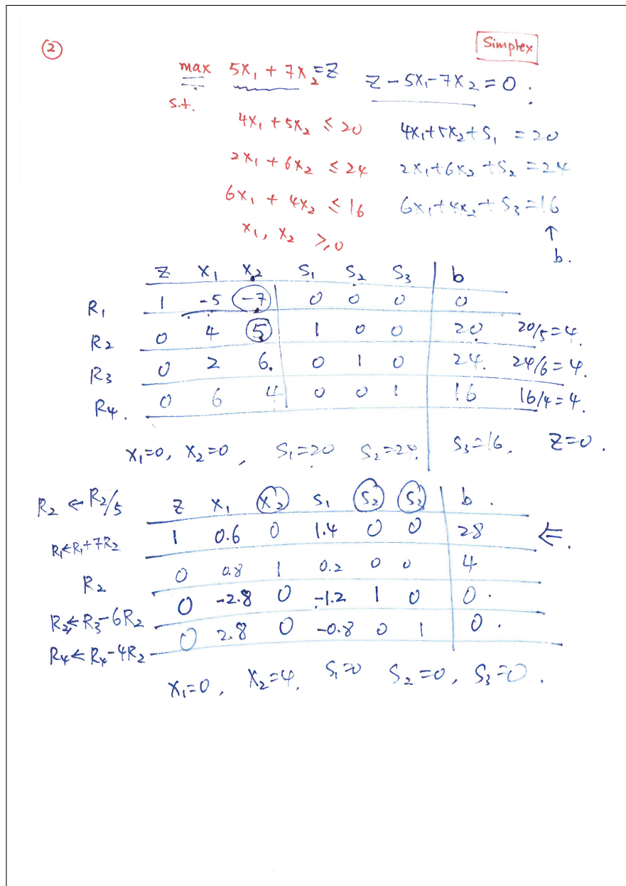
Figure 2: Q2 simplex on the same LP: three-way ratio-test tie, degenerate optimal tableau, z = 28 .
