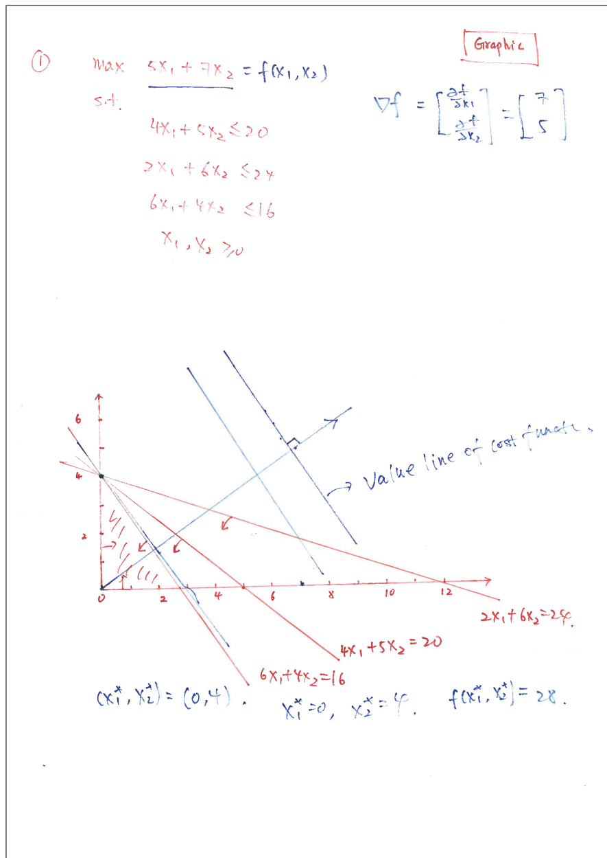
Figure 1: Q1 graphical: \max 5x_1 + 7x_2 s.t. 4x_1 + 5x_2 \leq 20 , 2x_1 + 6x_2 \leq 24 , 6x_1 + 4x_2 \leq 16 \Rightarrow (0, 4) , f = 28 (degenerate — all three lines through the optimum).
