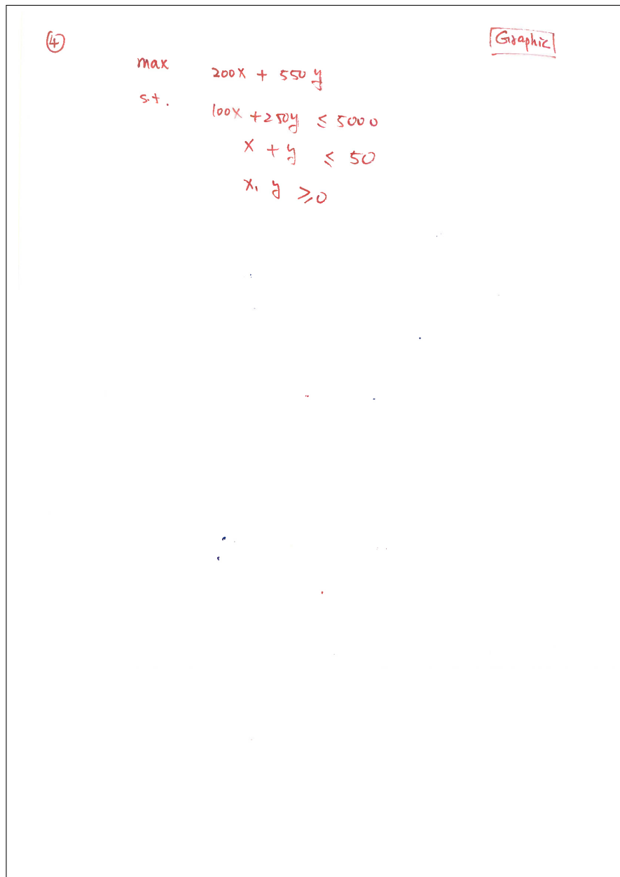
Figure 4: Q4 graphical: \max 200x + 550y s.t. 100x + 250y \leq 5000 , x + y \leq 50 \Rightarrow (0, 20) , value 11000.
