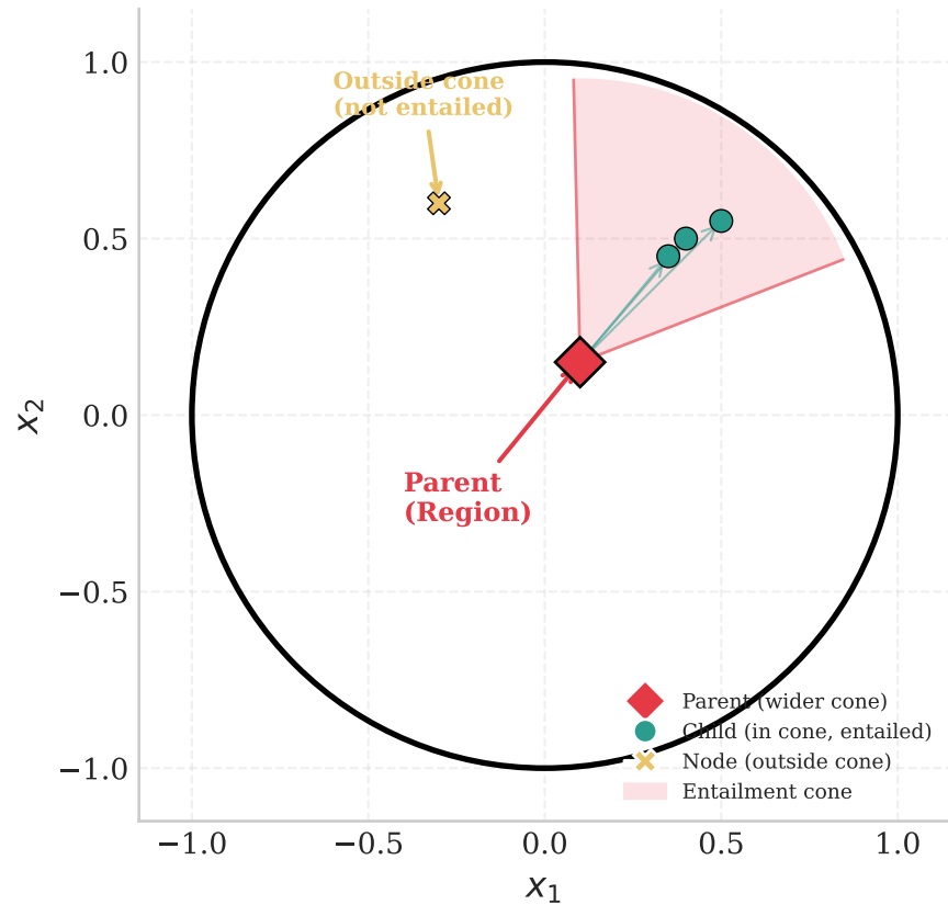
(b) Entailment Cone in Hyperbolic Space
