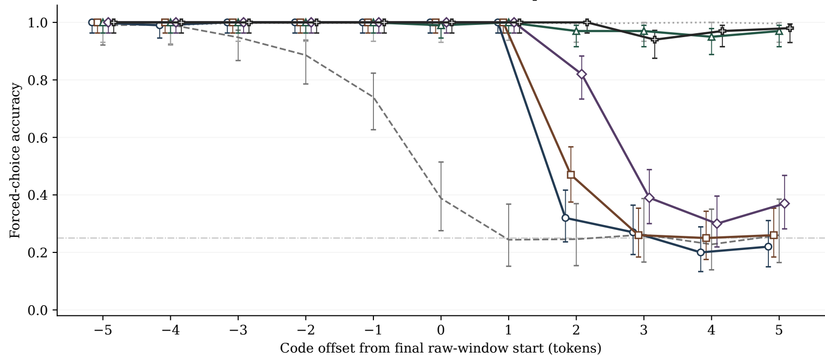
Secret-code retrieval · W = 512 · 100 trials per model and offset
