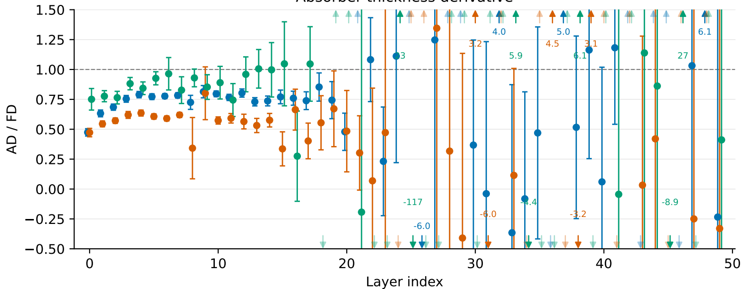
Absorber thickness derivative
