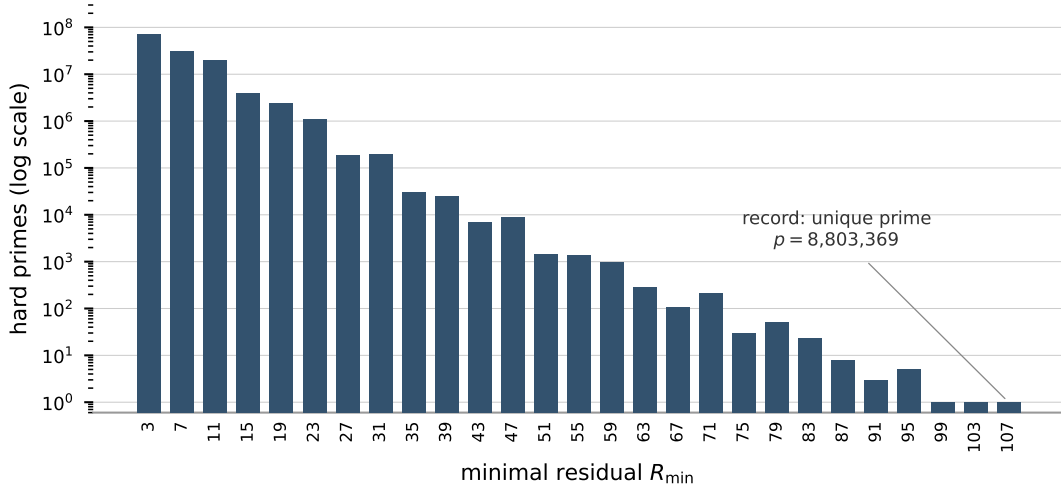
Figure 1: Distribution of the minimal residual R_{\min} over the 128,671,219 hard primes below 10^{11} (logarithmic count scale). The head is dominated by R = 3, 7, 11 ; the tail thins geometrically; the record R = 107 is attained by a single prime below 10^7 .
