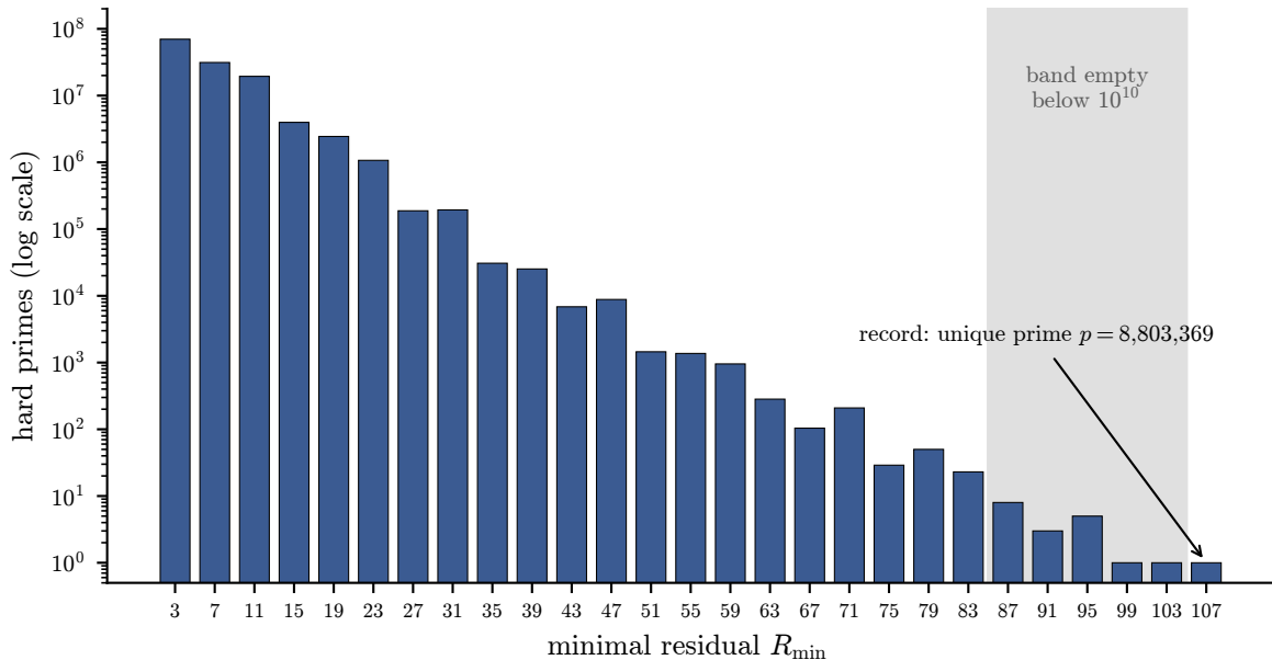
Figure 1: The data of Table 1 on a logarithmic count scale. The head is dominated by R = 3, 7, 11 ; the tail thins geometrically; the shaded band 87–103 was empty below 10^{10} and its late population matched the calibrated prediction (Section 5); the record R = 107 is attained by a single prime below 10^7 .
